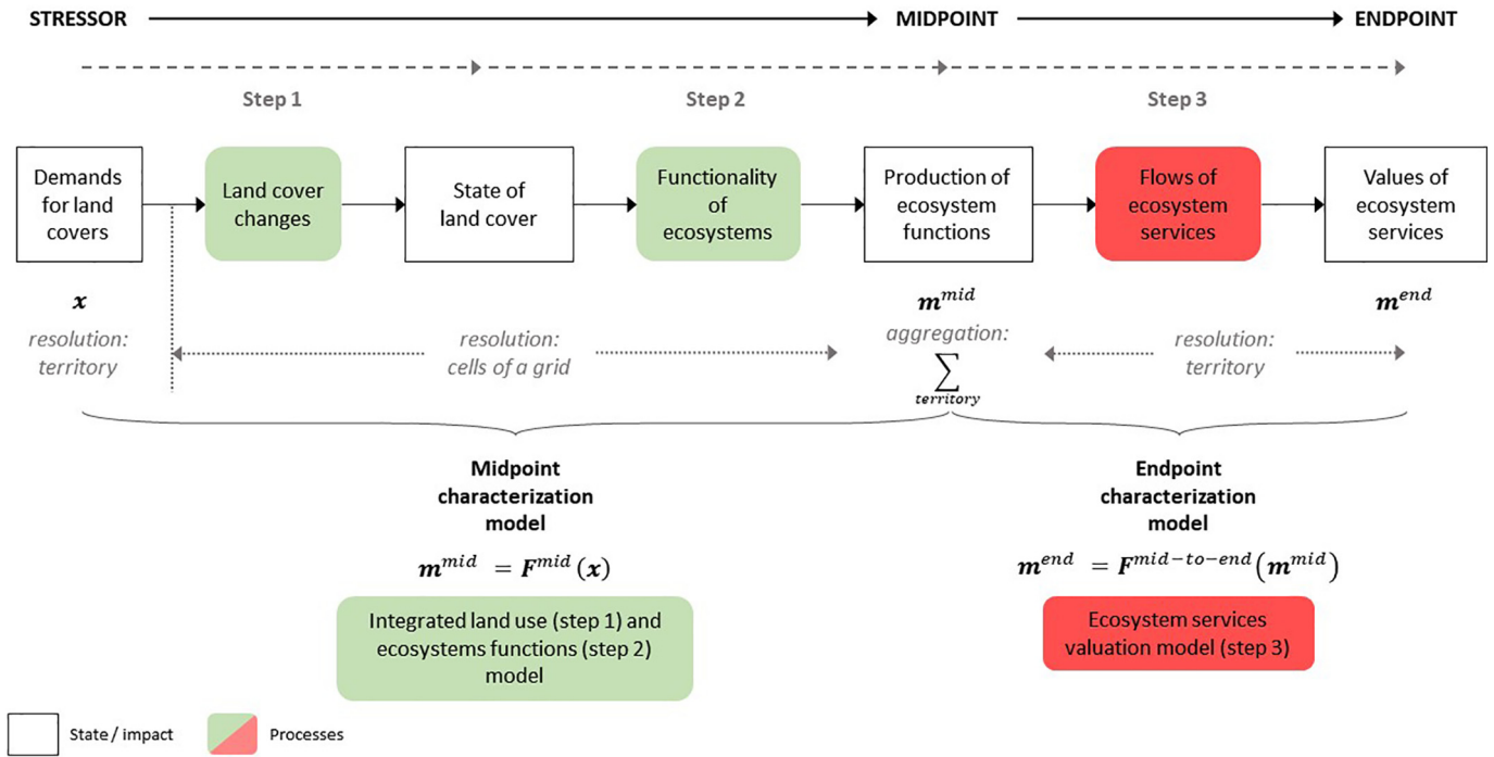
Fig. 1. Three-step cause-effect chain from demands for land covers (stressor \mathbf{x} that is accounted for in life cycle inventory) to the values of ecosystem services (endpoint indicator \mathbf{m}^{end} ). The bottom part represents the characterization models ( \mathbf{F}^{mid} and \mathbf{F}^{mid-to-end} ) that were implemented to simulate the midpoint and endpoint impacts in this paper. We consider the total production over a territory of ecosystem functions ( \mathbf{m}^{mid} ) and values of ecosystem services ( \mathbf{m}^{end} ) as midpoint and endpoint indicators, while we rely on the simulation of land cover and ecosystem functions at a higher resolution (cells of a grid). Rectangles denote states or impacts, rounded colored rectangles denote processes that connect such states, green represents the part between stressor and midpoint, red represents the part between midpoint and endpoint. (For interpretation of the references to colour in this figure legend, the reader is referred to the web version of this article.)
