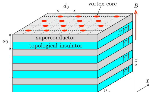
Figure 4.1: Cross-section through a heterostructure of alternating topological insulator layers and superconducting spacer layers. A perpendicular magnetization \beta separates a pair of Weyl cones of opposite chirality along k_z . Each Weyl cone is twofold degenerate in the electron-hole degree of freedom, mixed by the superconducting pair potential \Delta_0 . The mixing leaves the Weyl cones gapless, as long as the pair potential \Delta_0 remains smaller than \beta .
