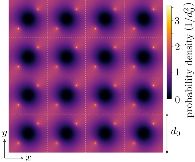
Figure 2.4: Color scale plot of |\psi(x, y)|^2 in the zeroth Landau level of the Weyl superconductor 9 . The white dashed lines indicate the vortex array, with a pair of h/2e vortices in each unit cell. On approaching a vortex core, when the separation \delta r \rightarrow 0 , the density diverges as a power law |\psi|^2 \propto \delta r^{1/\sqrt{2}-1} , in accord with Eq. (2.13).
