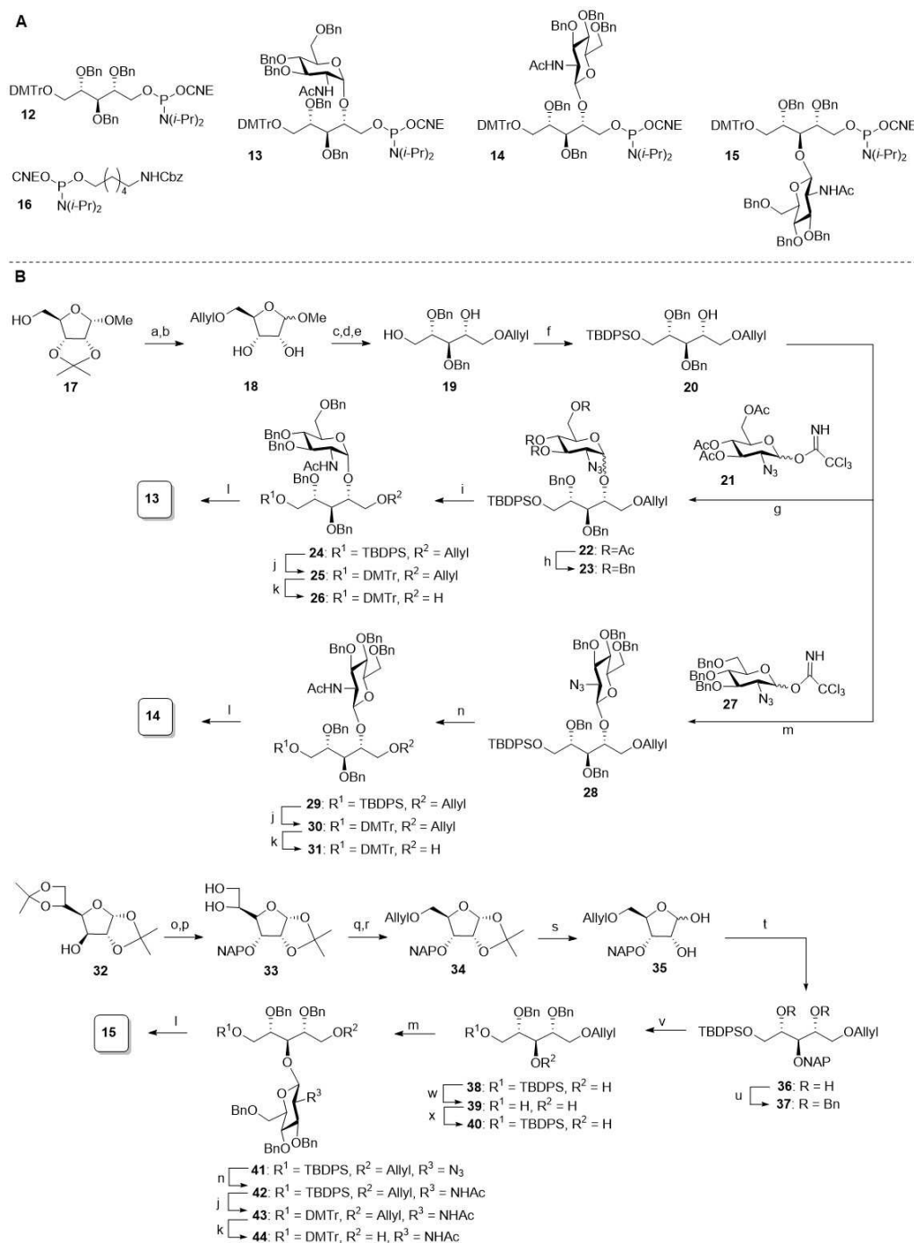
Scheme 1. Assembly of building blocks. a) AllylBr, NaH, THF/DMF (7:1), 0 °C to rt; b) AcOH/H 2 O 1:1, 50 °C, 300 mbar, 62 % over 2 steps; c) BnBr, NaH, THF/DMF (7:1), 0 °C to rt; d) 4 M HCl dioxane, 80 °C; e) NaBH 4 , MeOH, 0 °C, 50 % over 3 steps; f) TBDPSCI, TEA, DCM 0 °C to rt, 95 %. g) 21 , TMSOTf, DCM, rt, 92 %, 7:1 \alpha/\beta ; h) i. NaOMe, MeOH, rt, 70 % \alpha -anomer; ii) BnBr, NaH, THF/DMF (7:1), 0 °C to rt, 73 %; i) i . PMe 3 , KOH, THF; ii. Ac 2 O, pyridine, 24 : 89 % over 2 steps; j) i. TBAF, THF, rt; ii) DMTrCl, TEA, DCM, 25 : 67 %; 30 : 36 %; 43 : 60 %; k) i. Ir(COD)(Ph 2 MeP) 2 PF 6 , H 2 , THF, ii. I 2 , sat. aq. NaHCO 3 , THF, 26 : 88 %; 31 : 79 %; 44 : 94 %; l) 2-cyanoethyl- N,N -diisopropylchlorophosphoramidite, DIPEA, DCM, 13 : 81 %; 14 : 78 %; 15 : 85 %; m) 27 , TMSOTf, ACN, −40 °C to 0 °C, 28 : 85 %; 41 : 80 %; n) propanedithiol, pyridine, H 2 O, TEA, rt; ii. Ac 2 O, pyridine, 29 : 59 % 2 steps; 42 : 86 %; o) i. DMSO, Ac 2 O; ii. NaBH 4 , EtOH/H 2 O, 69 % over 2 steps; iii. NAPBr, NaH, TBAL, THF; p) p -TsOH·H 2 O, MeOH, 75 % over 2 steps; q) i. 0.2 M NaOAc in H 2 O, ethylene glycol, MeOH; ii. NaBH 4 , MeOH; r) AllylBr, NaH, THF/DMF, 88 %; s) THF/H 2 O/formic acid, 85 %; t) i. NaBH 4 , MeOH; ii. TBDPSCI, TEA, DCM, 57 % over 2 steps; u) BnBr, NaH, THF/DMF; v) DDQ, DCM/H 2 O; w) TBAF, THF, 62 % over 2 steps; x) TBDPSCI, TEA, DCM, 98 %.
