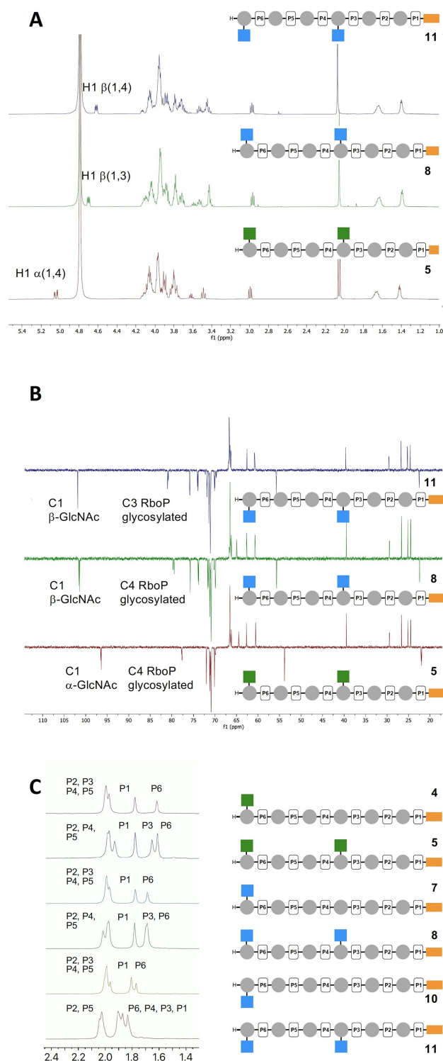
Figure 3. Characterization of the synthetic WTA-fragments. A) ^1\text{H} NMR (500 MHz, \text{D}_2\text{O} ) of 5, 8 and 11. B) ^{13}\text{C} NMR (126 MHz, \text{D}_2\text{O} ) of 5, 8 and 11. C) ^{31}\text{P} NMR (202 MHz, \text{D}_2\text{O} , 10 mg/mL, pH 7) of 4, 5, 7, 8, 10 and 11.
