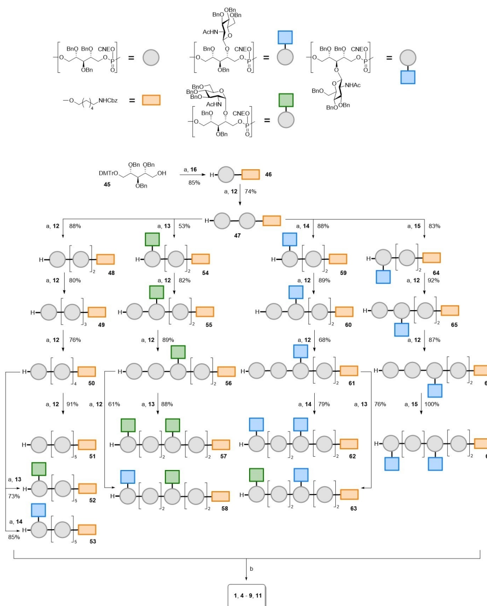
Scheme 2. Assembly of the target WTA-oligomers. Reagents and conditions: a) i. DCl, ACN, phosphoramidite 12 , 13 , 14 or 15 ; ii. CSO; iii. 3% DCA in DCM. b) i. \text{NH}_3 (30–33% aqueous solution), dioxane; ii. Pd black, \text{H}_2 , AcOH, \text{H}_2\text{O} /dioxane; 1 : 87%; 4 : 96%; 5 : 55%; 6 : 16%; 7 : 68%; 8 : 78%; 9 : 88%; 11 : 70%.
