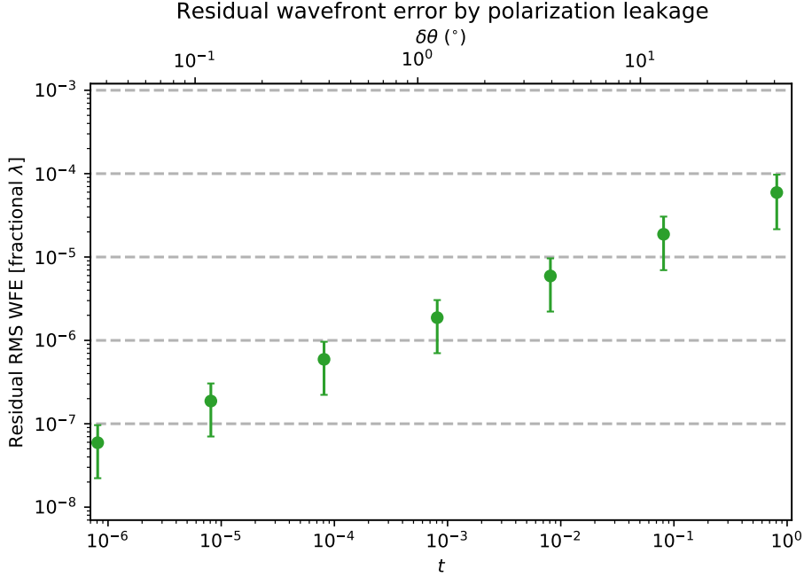
Figure 5.10: Performance of the wavefront sensing with polarization leakage. The error bars show the 1\sigma deviation over the 100 random wavefront aberration instances. The bottom x-axis shows polarization leakage ( t ), and the upper x-axis shows the equivalent rotation offset ( \delta\theta ) between the RH polarizer and PBS. We note that the right most data point is sampled at t = 0.81 .
