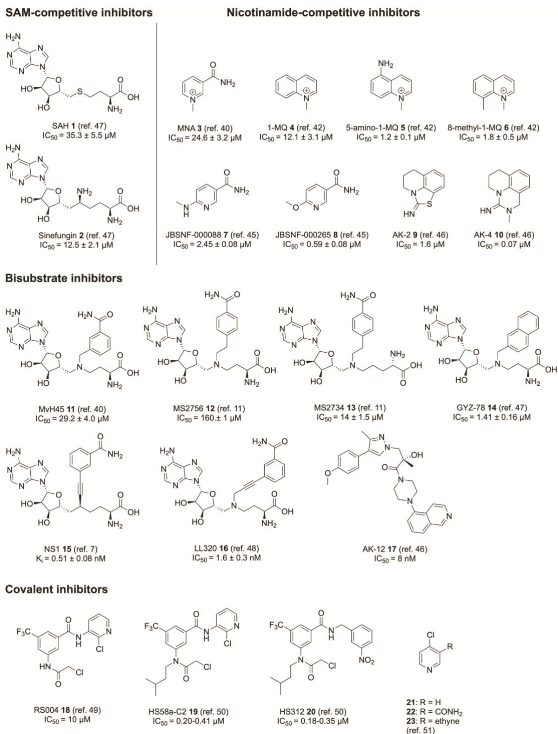
Figure 2. Overview of the chemical structures of nicotinamide N-methyltransferase (NNMT) inhibitors, including methyltransferase-specific inhibitors 1 and 2 , 47 nicotinamide-competitive inhibitors 3–10 , 40,42,45,46 bisubstrate inhibitors 11–17 , 7,11,40,46–48 and covalent inhibitors 18–23 . 49–51
