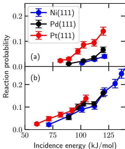
FIGURE 9.2: Reaction probability of \text{CHD}_3 on Ni(111) (blue), Pd(111) (black) and Pt(111) (red) for laser-off (a) and \nu_1 = 1 (b) using BOMD simulations. Results for Ni(111) and Pt(111) are taken from Refs. [12] and [13], respectively. The error bars represent 68% confidence intervals.
