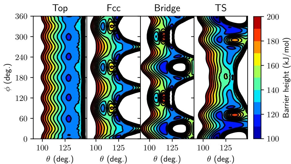
FIGURE 3.D.2: Barrier height of HCl on Au(111) as a function of the \theta and \phi angles for the top, fcc and bridge sites, and the minimum TS. The black contour lines are drawn at a interval of 10 kJ/mol from 100 to 200 kJ/mol.
