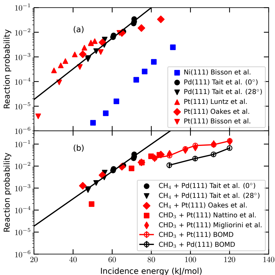
FIGURE 9.9: (a) Experimental reaction probability of \text{CH}_4 on \text{Ni}(111) (blue), \text{Pd}(111) (black) and \text{Pt}(111) (red) under laser-off conditions. Results for \text{Ni}(111) and \text{Pt}(111) are taken from Ref. [73] and Refs. [73–75], respectively. The \text{Pd}(111) results (black circles and triangles) are taken from Ref. [23], where the circles and triangles indicate an incidence angle of 0^\circ and 28^\circ , respectively, and the black line is a linear regression fit those points. (b) The reaction probability of \text{CH}_4 and \text{CHD}_3 on \text{Pd}(111) and \text{Pt}(111) obtained with experiment (closed symbols) and BOMD (open symbols) under laser-off conditions. For \text{CH}_4 + \text{Pt}(111) only the results from Ref. [75] are shown. The red squares and diamonds indicate results for \text{CHD}_3 + \text{Pt}(111) taken from Refs. [16] and [13], respectively.
