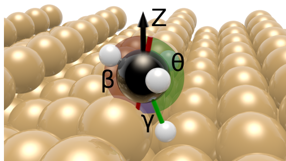
FIGURE 7.2: Methane on Cu(211) with the E/BtoB geometry, indicating the geometry angles as used in Table 7.2. \theta is the angle between the dissociating CH-bond and the surface normal, \beta is the angle between the umbrella axis and the surface normal, and \gamma is the angle between \theta and \beta .
