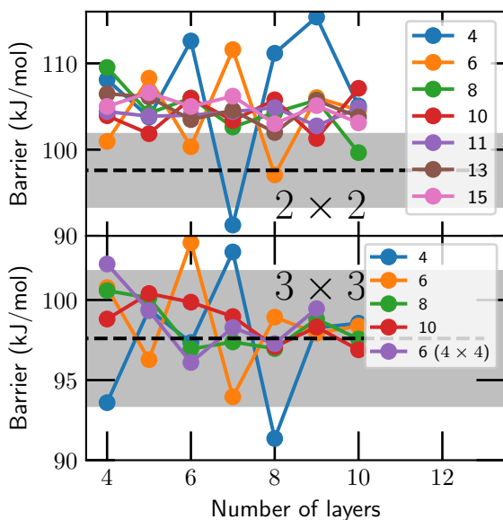
FIGURE 3.A.1: Convergence of the minimum barrier height (kJ/mol) of HCl on Au(111) as a function of the amount of layers and k -points using the MS-RPBE1 DF. The upper panel and lower panel used a 2 \times 2 and 3 \times 3 supercell, respectively. The second panel also includes the convergence for a 4 \times 4 supercell using a 6 \times 6 \times 1 k -point grid. The dashed lines indicate the converged barrier height. The calculations of the PES were done with a 3 \times 3 surface unit cell, 4 layers, and an 8 \times 8 \times 1 k -point grid. The amount of k -points is indicated in the legend.
