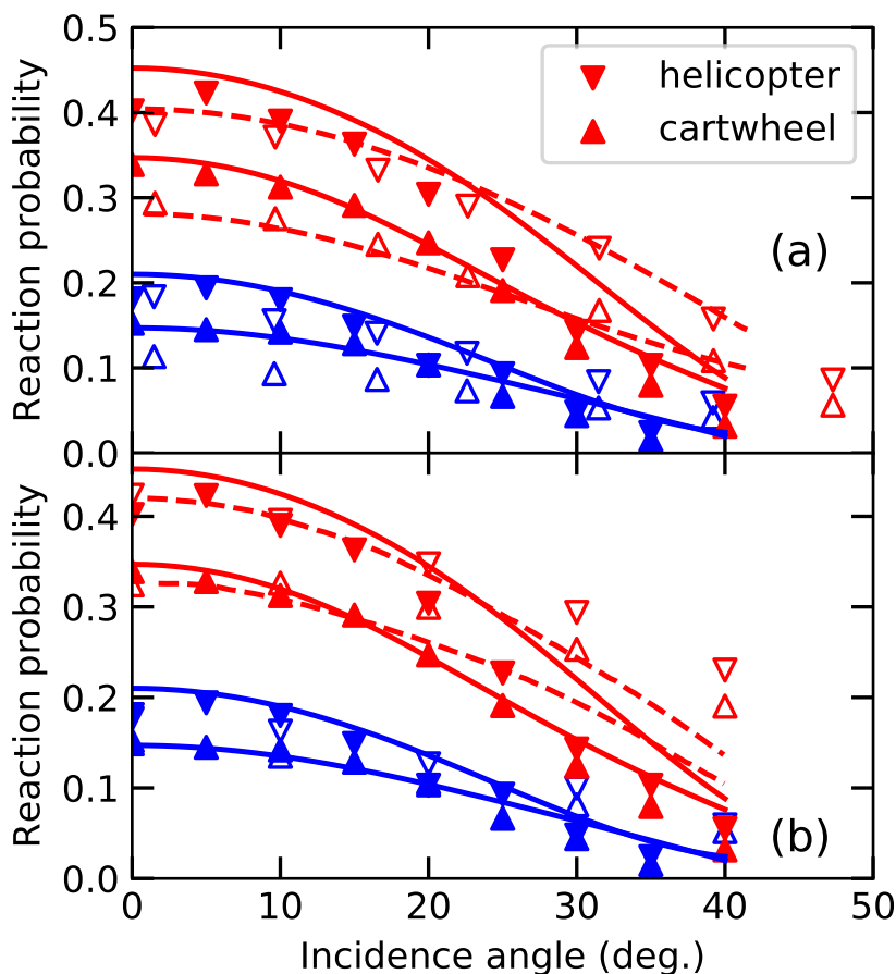
FIGURE 5.B.3: Sticking probability of O_2 ( v = 0, J = 2, K = 1 ) on Al(111) as a function of incidence angle (degrees). (a) The solid symbols and lines indicate results obtained with the HSE03-1/3X DF for E_i = 8.2 kJ/mol (blue) and E_i = 11.1 kJ/mol (red). The open symbols and dashed lines indicate results from experiment[65] for E_i = 9.6 kJ/mol (blue) and E_i = 17.4 kJ/mol (red). The downward and upward pointing triangles correspond to the helicopter and cartwheel orientations, respectively. The lines correspond to results obtained with the assumption of normal energy scaling. (b) Same as panel a, but instead of experimental results, the results from a FPLEPS PES based on ECW data[64] for E_i = 14.5 kJ/mol (blue) and E_i = 22.2 kJ/mol (red) are shown. In both cases, the incidence energies in the calculations have been chosen such that similar reaction probabilities are obtained in the calculations as in the experiments.
