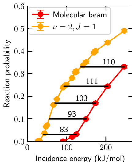
FIGURE 3.8: Sticking probability of HCl on Au(111) computed with the MS-RPBE DF. Results for a molecular beam with the initial rovibrational population according to the nozzle temperature (see Table 3.2) are indicated by the red circles, and the \nu = 2, j = 1 initial state selected results are indicated by the orange circles. Distances between the two curves along the energy axis are indicated by the horizon black lines and numbers (kJ/mol). The error bars represent 68% confidence intervals.
