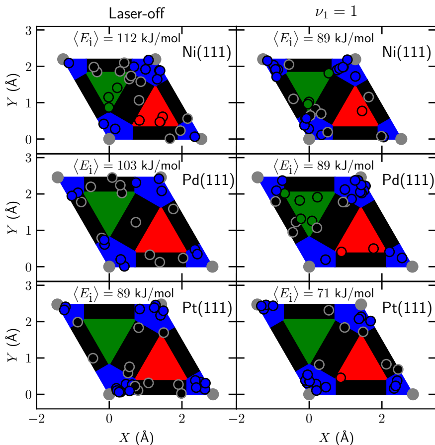
FIGURE 9.B.2: Impact site of reacting \text{CHD}_3 on Ni(111), Pd(111) and Pt(111) for laser-off and \nu_1 = 1 when a bond dissociates, i.e., r = r^\ddagger . Under laser-off conditions the reaction probability is about 2.5%, whereas for the \nu_1 = 1 conditions the reaction probability is about 5%. The top, fcc, hcp and bridge sites are indicated in blue, red, green and black, respectively, and the top layer atoms are indicate by the gray circles.
