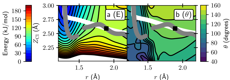
FIGURE 3.5: Elbow plots of HCl on Au(111) as a function of Z_{\text{Cl}} and r using the MS-RPBEI DF for the top site showing the energy (a, kJ/mol) and the \theta angle (b, degrees). All degrees of freedom other than Z_{\text{Cl}} and r are relaxed. Black contour lines are drawn at an interval of 10 kJ/mol between 0 and 200 kJ/mol (energy) or at an interval of 10^\circ between 40^\circ and 160^\circ ( \theta ). The grey circles indicate the MEP in reduced dimensionality and the black square indicates the highest point along the MEP. Note that the break along the MEP is an artifact caused by the procedure employed to obtain the MEP (see Figure 3.D.1). The white circles indicate the MEP as it is obtained conventionally using a steepest descent from the TS.
