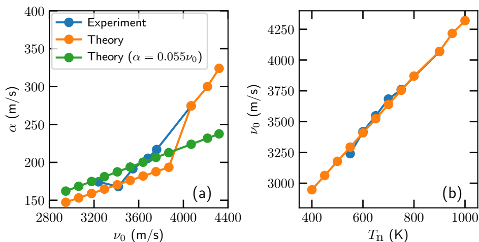
FIGURE 8.2: Width parameter \alpha as a function of the stream velocity v_0 (a) and the stream velocity v_0 as a function of the nozzle temperature T_n (b). Experimental parameters[9] and parameters used in this work are indicated in blue and orange, respectively. Theoretical parameters where \alpha = 0.055v_0 are indicated in green.
