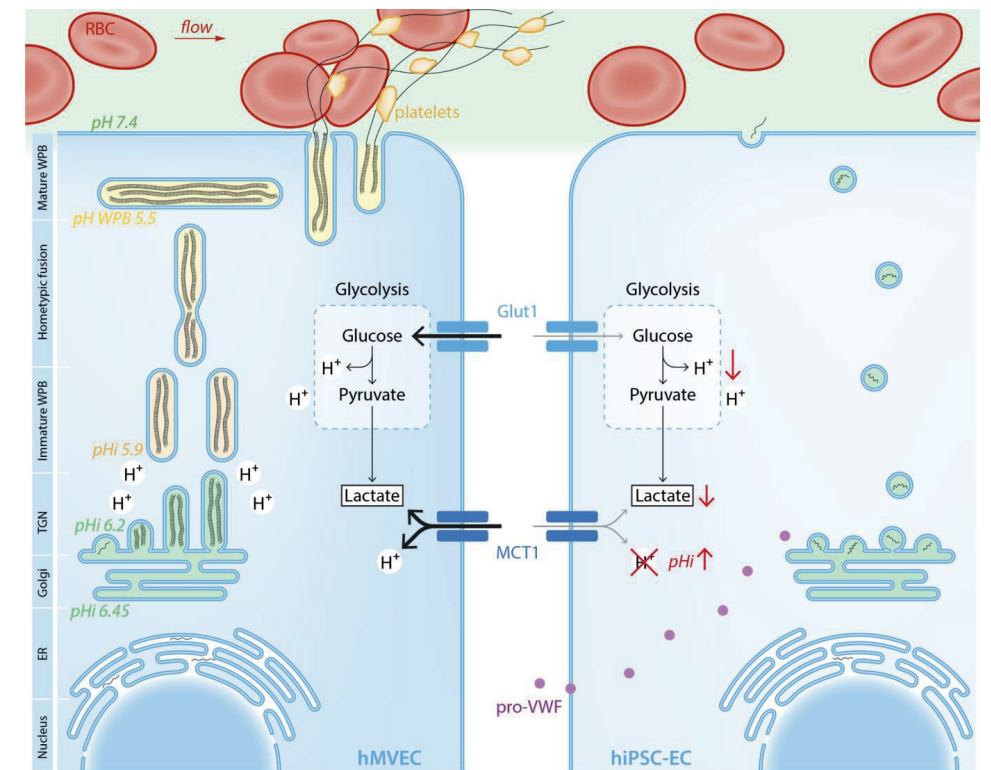
Figure 6. Schematic overview of WBP production and the metabolic regulation of pHi of hMVECs and hiPSC-ECs. Formation of mature WPB in hiPSC-ECs is limited by the increased intracellular pH around the Golgi apparatus and Trans Golgi Network (TGN). This increase in pHi is caused by reduced intracellular lactate accompanied by reduced H^+ , caused by reduced glycolysis and reduced uptake of lactate and H^+ via MCT1. This increased pHi limits intrachain disulphide bonds formation and association of the pro-peptide, after furin cleavage, with the mature VWF peptide at the trans-Golgi network (TGN) and WPB. Both dimeric bouquets formation and helical arrangement of VWF are pH regulated. Eventually this reduces the amount of WPB and limits the functionality of the endothelial cell.
