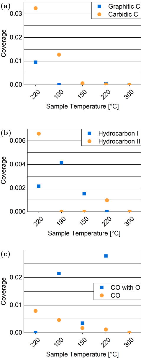
Figure 5.21: Results of the detailed fits of C 1s spectra measured in 0.25 mbar H 2 at different temperatures distinguishing (a) carbodic from graphitic C, (b) two types of hydrocarbons, and (c) CO alone from CO co-adsorbed with O.
