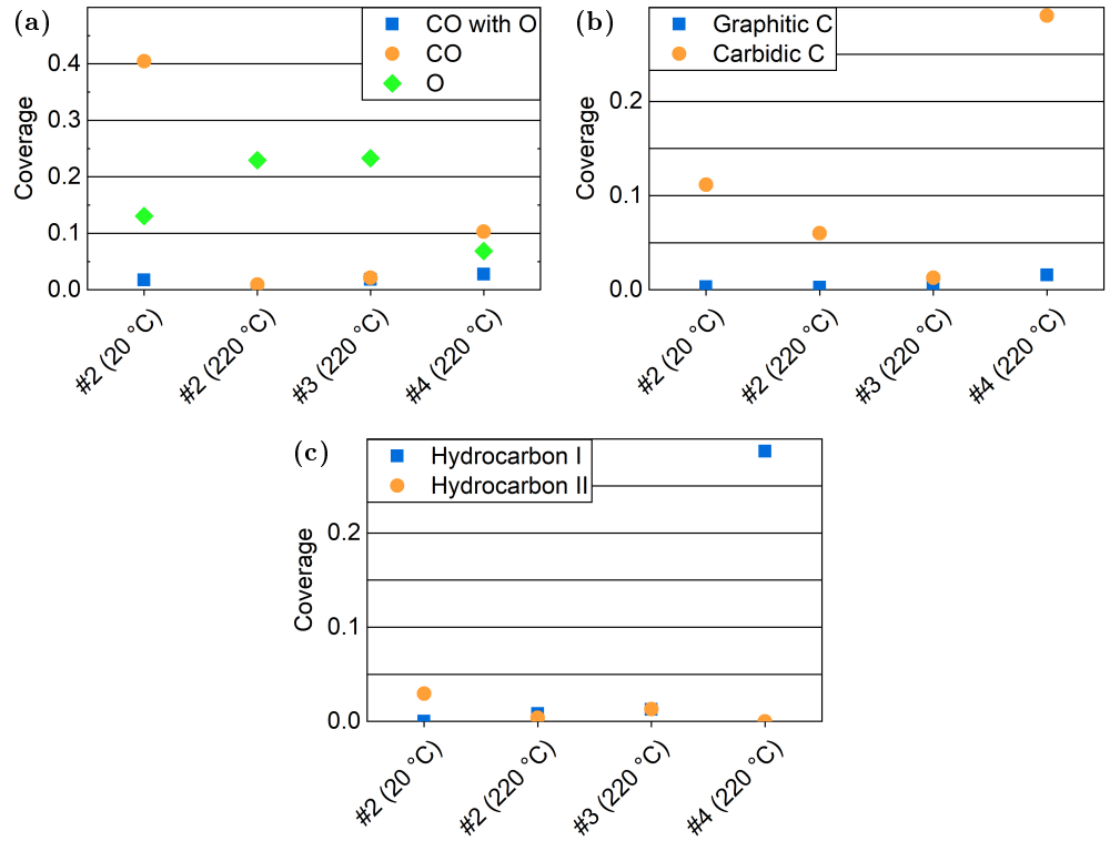
Figure 5.20: Results of the detailed fits of C 1s spectra measured on different as-prepared samples in UHV (a) distinguishing CO alone from CO co-adsorbed with O compared to the O coverage from the O 1s spectra, (b) distinguishing carbodic and graphitic C, and (c) distinguishing two types of hydrocarbons.
