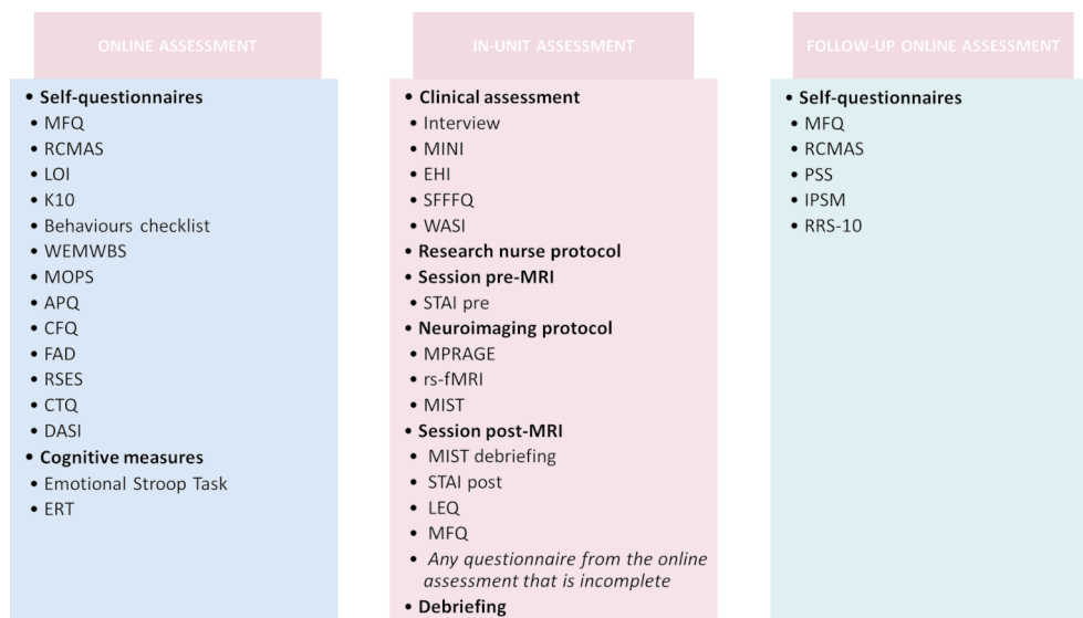
Figure 4 Summary of the study protocol. APQ, Alabama Parenting Questionnaire; CBC, Child Behaviours Checklist; CFQ, Cambridge Friendship Questionnaire; CTQ, Childhood Trauma Questionnaire; DASi, Drugs Alcohol and Self-Injury; EHI, Edinburgh Handedness Inventory; ERT, Emotion Regulation Task; FAD, Family Assessment Device; IPSM, Interpersonal Sensitivity Measure; K10, Kessler Psychological Distress Scale; LEQ, Life-Events Questionnaire; LOI, Leyton Obsessional Inventory; MFQ, Mood and Feelings Questionnaire; MINI, Mini-International Neuropsychiatric Interview; MIST, Montreal Imaging Stress Task; MOPS, Measure of Parenting Style; MPRAGE, T1-Weighted rapid three-dimensional gradient-echo; PSS, Perceived Stress Scale; RCMAS, Revised Children's Manifest Anxiety Scale; RRS-10, Ruminative Response Scale; RSES, Rosenberg Self-Esteem Scale; rs-fMRI, resting state functional MRI; SFFFQ, Short-Form Frequency Food Questionnaire; STAI, State-Trait Anxiety Inventory; WASI, Wechsler Abbreviated Scale of Intelligence; WEMWBS, Warwick-Edinburgh Mental Well-Being Scale.
