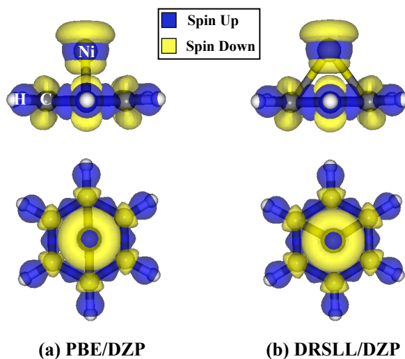
Figure 4.6: Side view and top view of spin density isosurface (isovalue 0.005 e/A 3 ) of Benz-Ni 2+ computed in triplet state at PBE/DZP and DRSLL/DZP level. Spin population and atomic labels are reported.
