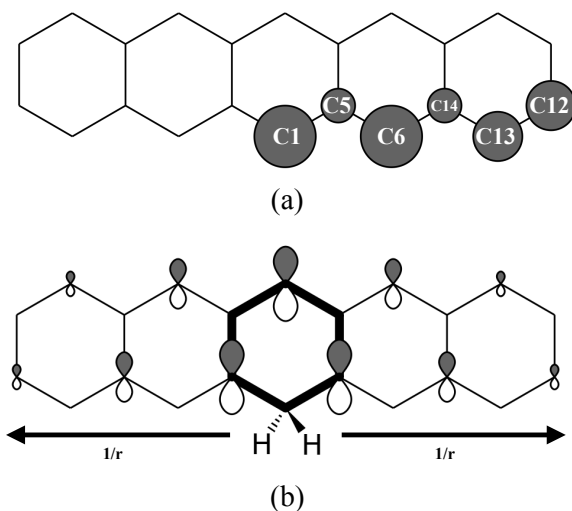
Figure 2.3: (a) Schematic representation of the affinity of the carbon atoms to be chemisorbed by the first hydrogen atom. Larger balls indicates higher hydrogenation affinity. (b) Graphical representation of localized mid-gap states for the second hydrogenation. The arrows show decreasing effect of mid-gap state with increasing distance from the first hydrogenated carbon site.
