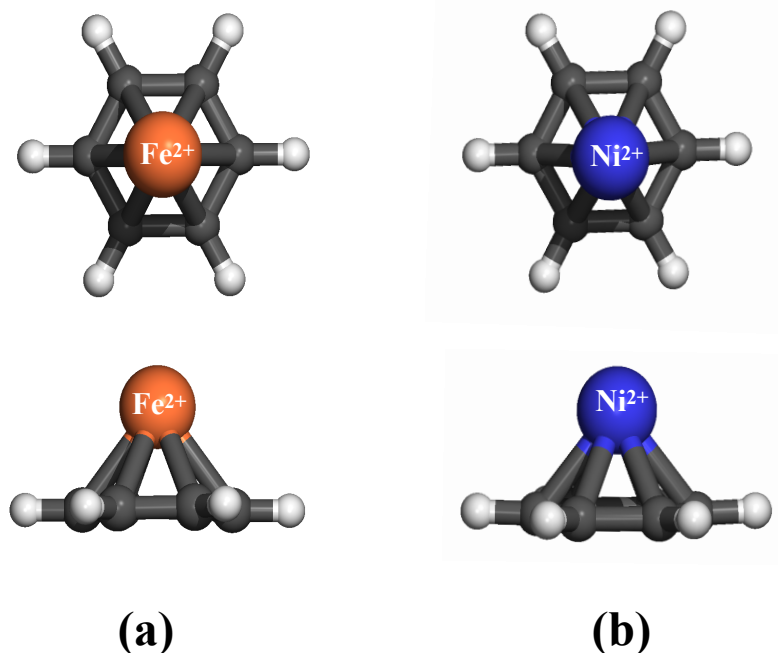
Figure 4.4: Top view and side view of the optimized geometry (PBE/DZP) of benzene coordinated with (a) \text{Fe}^{2+} (Benz- \text{Fe}^{2+} ) in quintet state and (b) \text{Ni}^{2+} (Benz- \text{Ni}^{2+} ) in triplet state.
