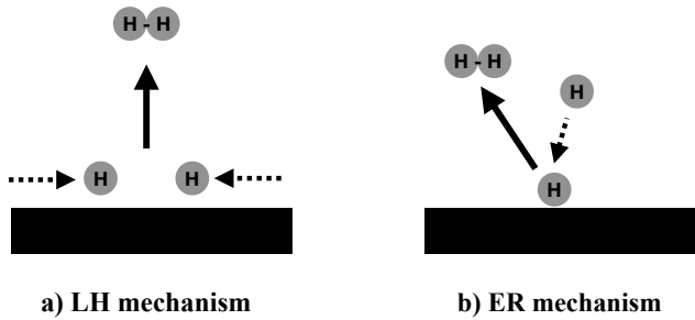
Figure 1.7: Schematic representation of molecular hydrogen formation through Langmuir–Hinshelwood (LH) and Eley–Rideal (ER) mechanism on a solid surface.
