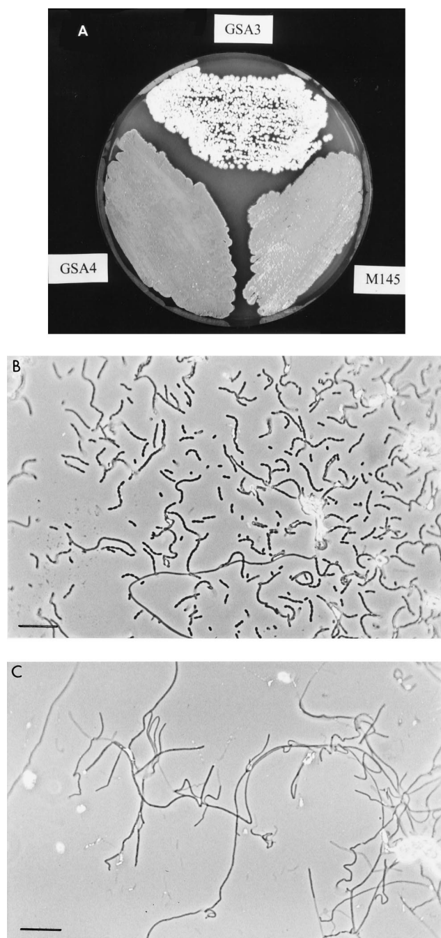
FIG. 4. (A) Phenotype of the ssg4 null mutant of S. coelicolor M145 on SFM medium. GSA3 is the ssg4 mutant of M145; GSA4 is the ssg4 mutant complemented with pGWS7. The white appearance of GSA3 is due to the failure of the mutant to produce the grey-pigmented spores. GSA4 consistently produces more spores than M145. (B and C) Impression prints of the surfaces of solid-grown cultures of S. coelicolor M145 (B) and its ssg4 null mutant GSA3 (C). While M145 sporulates abundantly, aerial hyphae of GSA3 show typical coiling, but no spores (bars = 10 \mu m).
