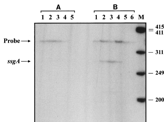
FIG. 5. Transcriptional analysis of ssgA . (A) Analysis of samples taken from normal growth curve in MM. Lanes 1 to 5 refer to samples taken at an OD 550 of 0.3 (early log), 0.6 (mid-log), 0.9 (late log), 1.2 (transition phase), and 1.5 (stationary phase), respectively. (B) Analysis of samples taken after nutritional shift-down. Lanes 1 to 6 refer to samples taken 0, 15, 30, 60, 120, and 240 min after shift-down, respectively. Lane M, 32 P-end-labeled Hae III-digested \phi X174 size markers; numbers on the right refer to sizes of the marker bands (in nucleotides). Positions of the ssgA transcript and reannealed probe are shown on the left.
