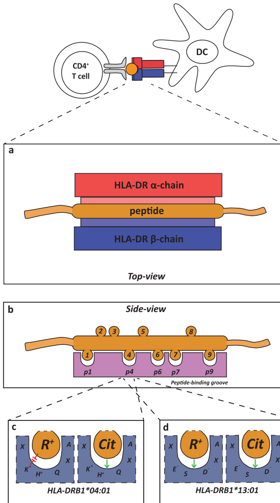
Figure 1: Schematic representation of a peptide binding to a HLA-DR molecule
