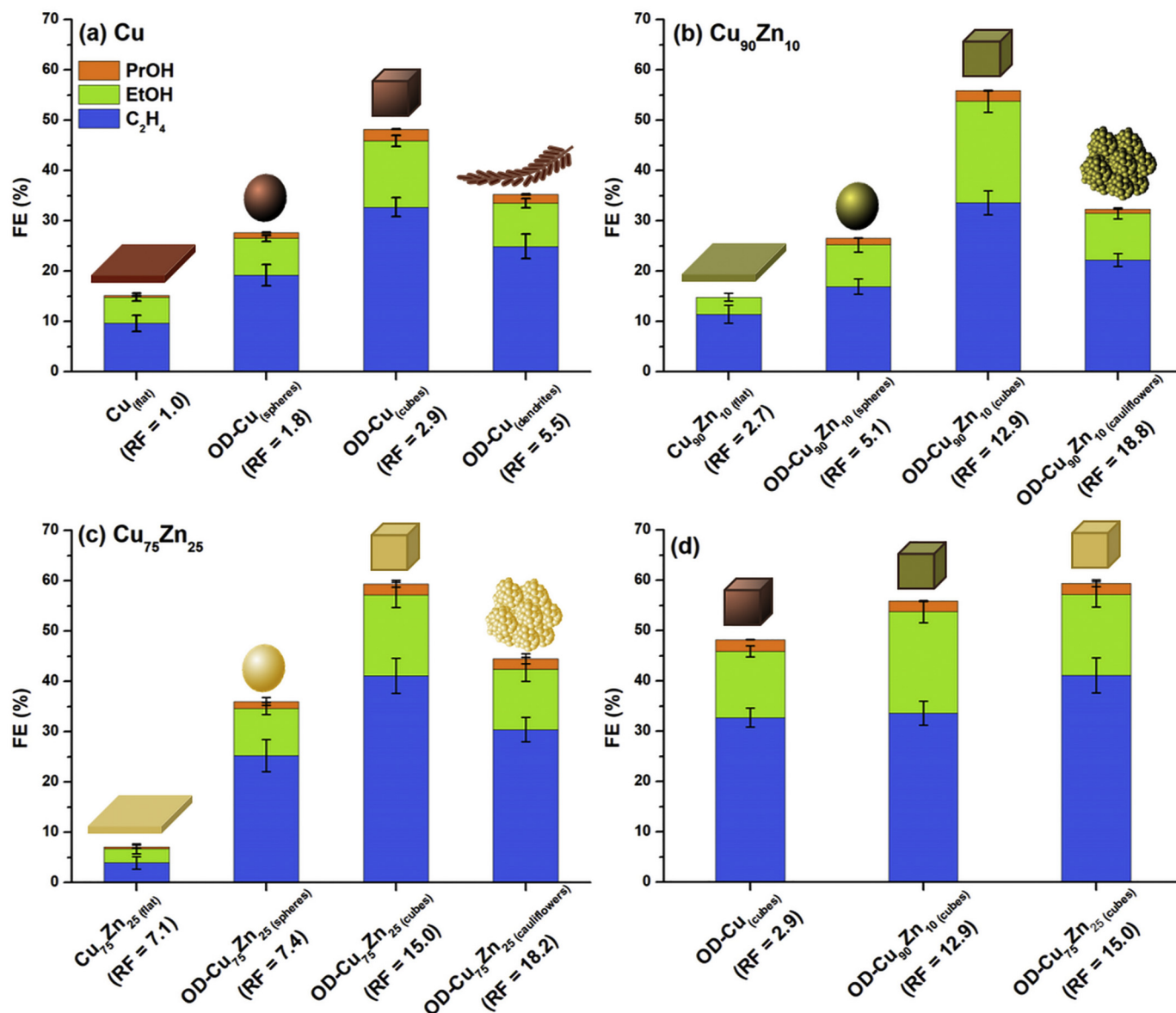
Fig. 3. Faradaic efficiency (FE) of the C 2 H 4 (blue), EtOH (green), and PrOH (orange) production on (a) Cu (flat) , OD-Cu (spheres) , OD-Cu (cubes) , and OD-Cu (dendrites) , (b) Cu 90 Zn 10 (flat), OD-Cu 90 Zn 10 (spheres), OD-Cu 90 Zn 10 (cubes), and OD-Cu 90 Zn 10 (cauliflowers), (c) Cu 75 Zn 25 (flat), OD-Cu 75 Zn 25 (spheres), OD-Cu 75 Zn 25 (cubes), and OD-Cu 75 Zn 25 (cauliflowers), and (d) OD-Cu (cubes) , OD-Cu 90 Zn 10 (cubes), and OD-Cu 75 Zn 25 (cubes) at -1.1 V vs RHE. Roughness factor (RF) values were added below the name of each electrode to facilitate the discussion. (For interpretation of the references to color in this figure legend, the reader is referred to the web version of this article.)
