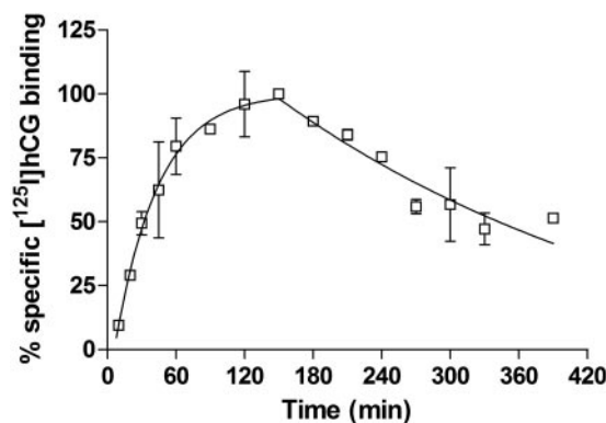
Fig. 4. Association and dissociation kinetics of 125 I-hCG binding to CHO-K1 membranes expressing the human luteinizing hormone receptor at 30°C. Representative graphs from one experiment performed in duplicate (see Table 1 for kinetic parameters).
