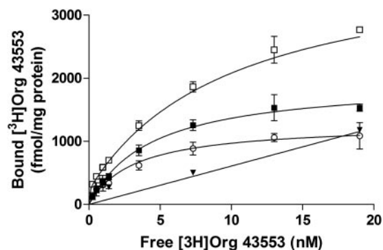
Fig. 2. Saturation of [ 3 H]Org 43553 to luteinizing hormone receptors in the absence (control) or presence of 70 nM recLH. The control specific binding (■) was determined by subtracting the nonspecific binding (▼) from the total binding (□) curve. The control K D value was 2.4 ± 0.4 nM and the B max value was 1.6 ± 0.2 pmol/mg protein ( n = 5). A similar experiment was performed in the presence of 70 nM recLH, of which only the specific binding is shown (○). Representative graphs from one experiment performed in duplicate.
