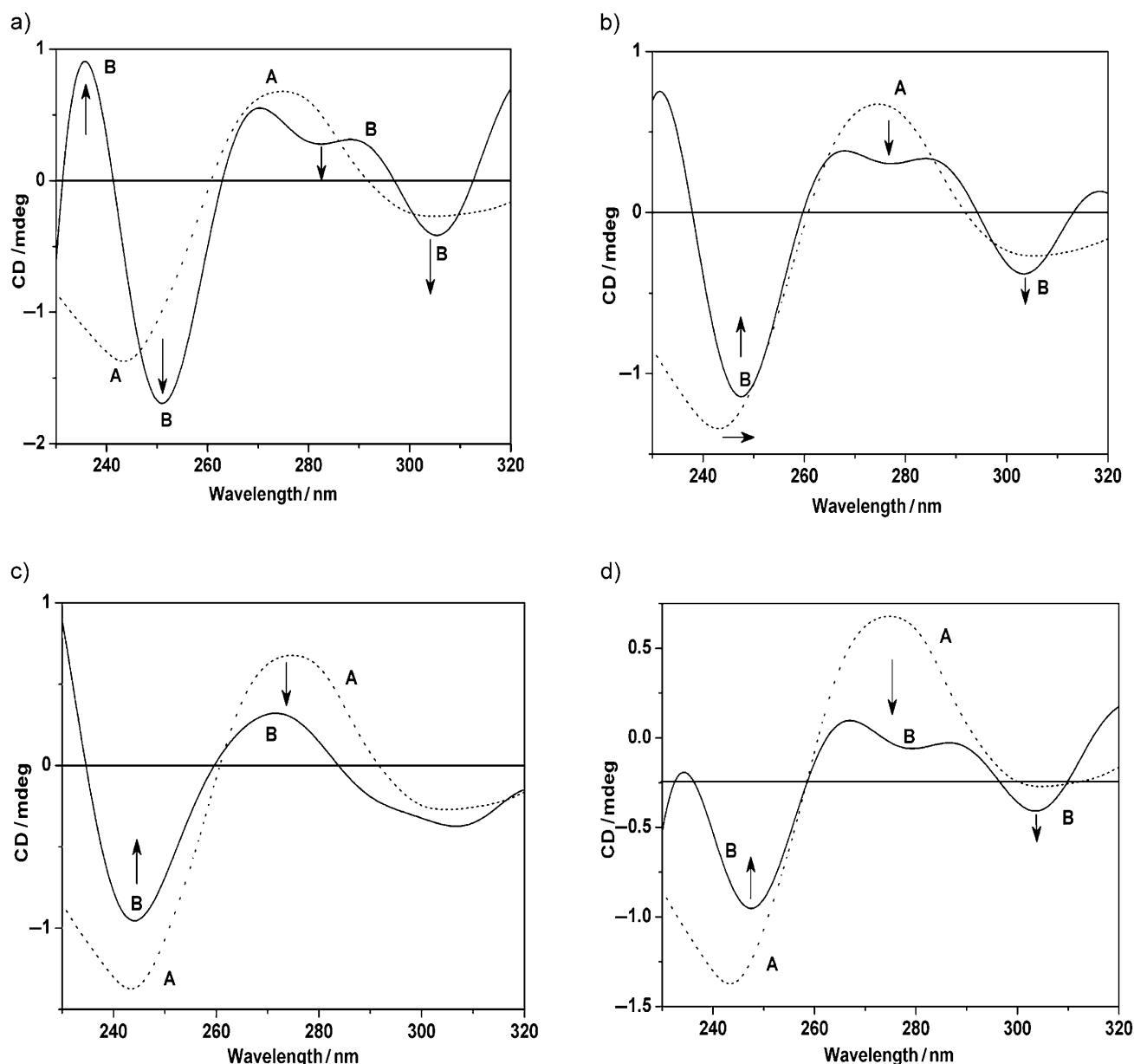
Figure 3. Circular dichroism for the analysis of the effect of a) phendione (L 1 ), c) dppz (L 2 ), and their Pt complexes b) and d), respectively, on the conformation of calf thymus DNA. Prominent changes in CD spectra were observed in relation to native DNA (trace A) induced by the ligands and their platinum complexes (trace B).
