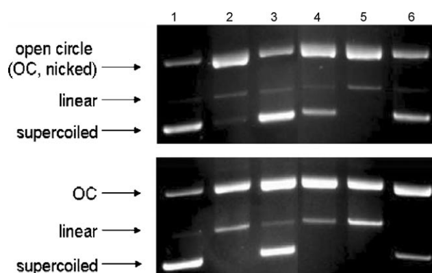
Figure 2. Agarose gel electrophoresis showing the effects of phenanthroline-type compounds on DNA integrity. All compounds were incubated at concentrations of 25 \mu M (top) or 100 \mu M (bottom), with 20 \mu M \phi X174 DNA (in base pairs). Reaction mixtures contained a 4:1:16 ratio of compound/CuSO 4 /ascorbic acid and were incubated for 30 min at 37 °C in the dark. Lane 1: DNA without added compound; lanes 2–6: DNA incubated with L 1 (2), [PtL 1 Cl 2 ] (3), L 2 (4), [PtL 2 Cl 2 ] (5), CuSO 4 (6.25 \mu M, top; 25 \mu M, bottom) and ascorbic acid (100 \mu M, top; 400 \mu M, bottom) (6).
