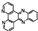
dipyrdo[3,2- \alpha :2',3'- c ]phenazine ( L^2 )
