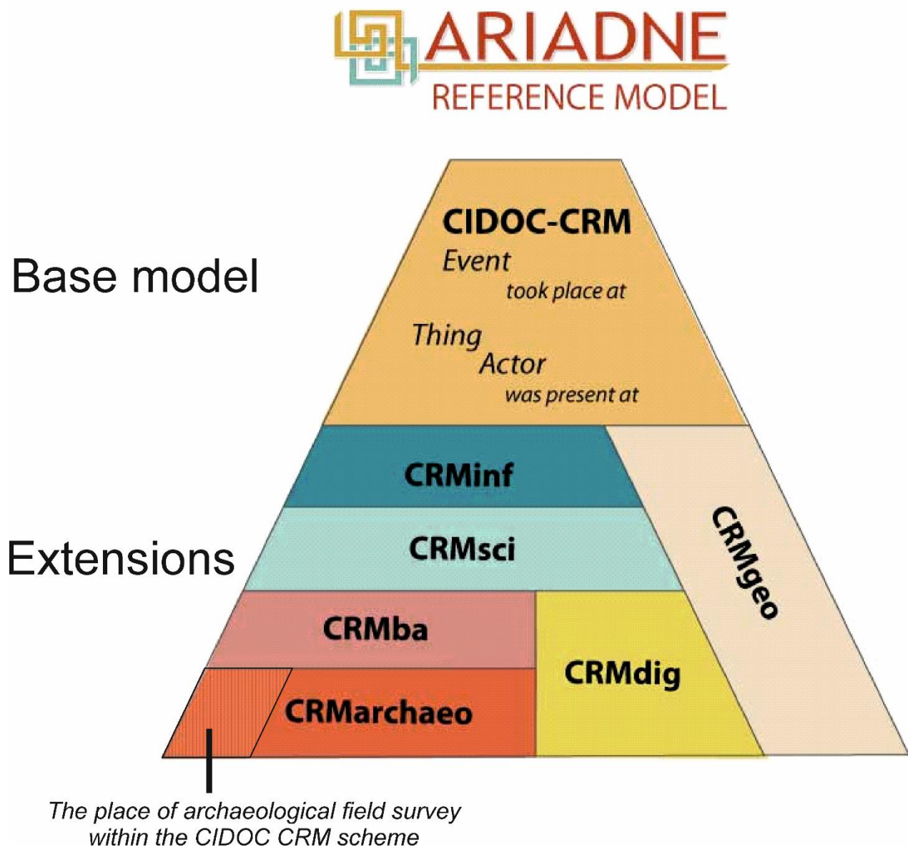
Fig. 1. The ARIADNE reference model (modified from https://www.ics.forth.gr/isl/index_main.php?l=e&c=229 ).
