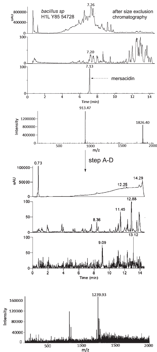
Scheme 3 Protocol for the two-step labeling of the lantibiotic mersacidin.
