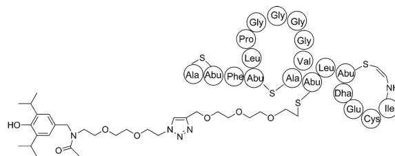
Scheme 4 Two-step labeling strategy for the identification of mersacidin from cultured Bacillus sp. H1L Y85 54728.
