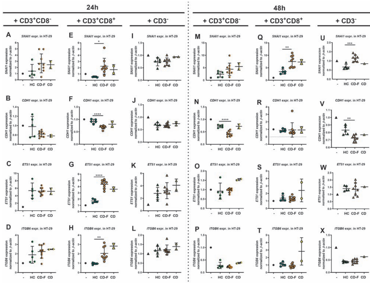
FIGURE 4. EMT-related gene expression in HT-29 monolayer co-cultured for 24 hours and 48 hours without leukocytes (-), or with sorted CD3 + CD8 - , CD3 + CD8 + or CD45 + CD3 - immune cells derived from HC, CD-F, or CD. After 24 hours of co-culture with CD3 + CD8 - cells, no significant changes in mRNA expression level of SNAI1 (A), CDH1 (B), and ITGB6 (D) were detectable between the 3 different groups. Only ETS1 was upregulated compared to untreated cells (C). After 24 hours of co-culture with CD3 + CD8 + cells, T cells from CD-F induced significant changes in SNAI1 (E), CDH1 (F), ETS1 (G), and ITGB6 (H) expression. 24 hours of co-culture with CD3 - cells revealed no significant changes (I–L). After 48 hours of co-culture with CD3 + CD8 - cells, T cells from CD-F showed a trend for higher SNAI1 expression (M) and significantly reduced CDH1 (N). CD3 + CD8 - cells from CD induced changes for ETS1 expression after 48 hours (O) and ITGB6 expression did not differ (P). Co-culture of CD3 + CD8 + cells for 48 hours induced enhanced SNAI1 expression with cells from CD-F (Q), whereas CDH1 expression showed no more differences between all groups (R). CD3 + CD8 + T cells from CD triggered increased expression of ETS1 (S) and ITGB6 (T) after 48 hours. After 48 hours of co-culture with CD3 - cells, gene expression differences were observed for SNAI1 (U) and CDH1 (V) but not for ETS1 (W) or ITGB6 (X). * P ≤ 0.05, ** P ≤ 0.01, *** P ≤ 0.001, and **** P ≤ 0.0001; - ( n = 1 for each condition), HC ( n = 5), CD-F ( n = 9 for CD3 + CD8 - and CD3 + CD8 + and n = 8 for CD3 - ), and CD ( n = 2 for CD3 + CD8 - [24 hours, 48 hours], CD3 + CD8 + [24 hours, 48 hours], and CD3 - [24 hours] and n = 1 for CD3 - [48 h]).
