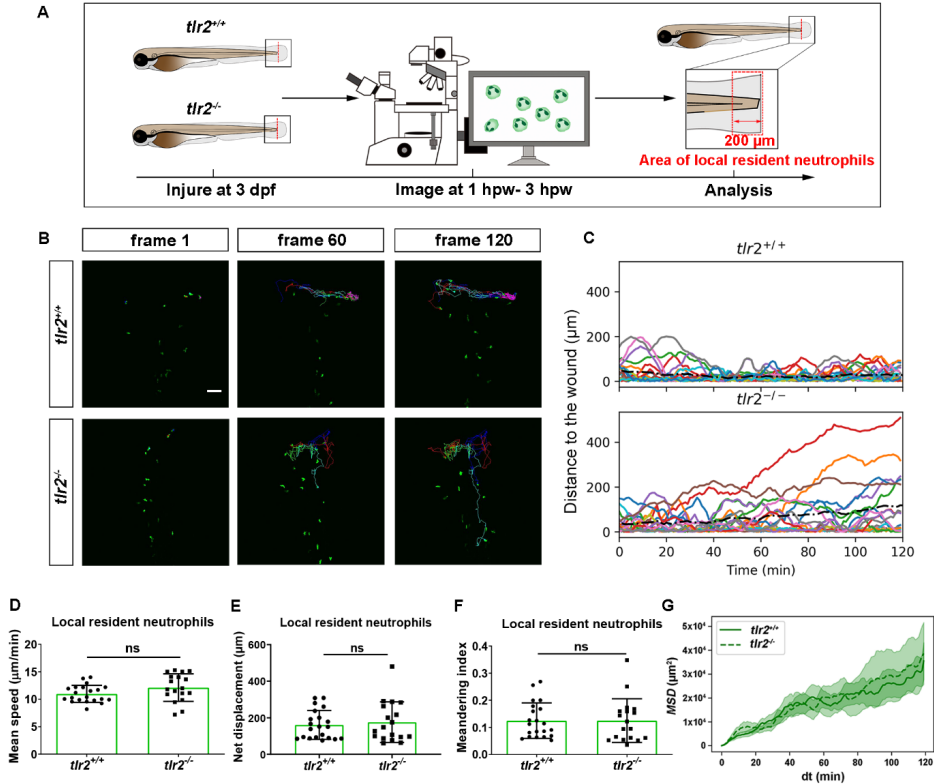
FIGURE 5.7: Quantification of localized resident neutrophils behavior in wounded tlr2 larvae. (A) Experimental scheme. (B) Representative images of local resident neutrophils tracks in the wounded tail fin of 3 dpf tlr2 +/+ or tlr2 -/- larvae at frame 1, frame 60 and frame 120. Cell tracking movies are shown in Supplementary Movie S17-18). Scale bar: 50 µm. (C) Distance to the wound. Black dash line represents average distance to the wound. Each color line represents one cell. (D-I) Quantification of local resident neutrophil tracks, mean speed (D); net displacement (E); Meandering index (F); MSD (G). An unpaired, two-tailed t-test was used to assess significance (ns, non-significance) and data are shown as mean±SD.
