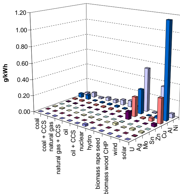
Fig. 3. Requirements of selected metals in different power generation technologies.
