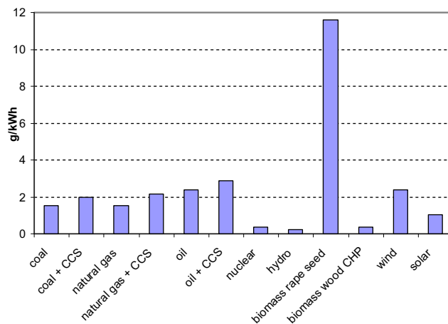
Fig. 2. Iron requirements in different power generation technologies.
