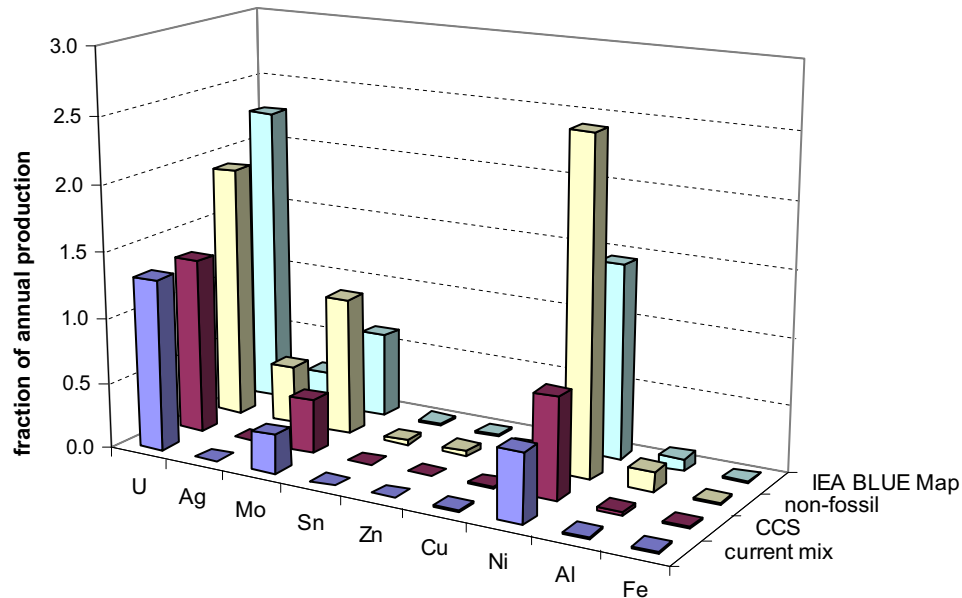
Fig. 8. Requirements of selected metals in different power mix cases compared with world annual mine production of these metals.
