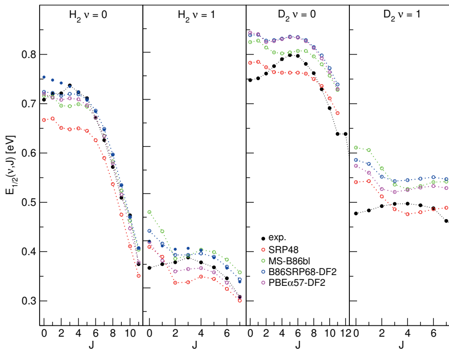
FIGURE 5.14: E_{1/2}(\nu, J) parameters as a function of J obtained using method A1 for \text{H}_2 and \text{D}_2 reacting on \text{Cu}(111) . Red circles represent the SRP48 values 63 , green circles the MS-B86bl values 13 , blue circles represent the B86SRP68-DF2 values with the solid blue circles corresponding to QD calculations, magenta circles represent the PBE \alpha 57-DF2 values, and solid black circles represent experimental results 48 .
