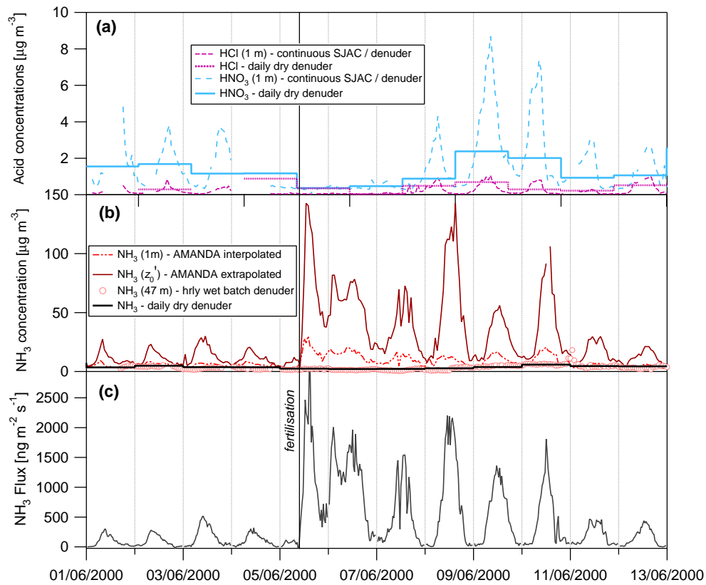
Fig. 2. Evolution of the gas concentrations of (a) HCl and HNO 3 and (b) NH 3 1 m and 47 m above the grassland, compared with the NH 3 concentration extrapolated to the canopy (NH 3 ( z_0' )). (c) Flux of NH 3 . The fertilizer was applied on 5 June 08:00 to 10:00 GMT. The concentrations and fluxes of NH 3 are based on the best estimate \chi_{\text{NH}_3} and F_{\text{NH}_3} provided by Milford et al. (2008). See text for details.
