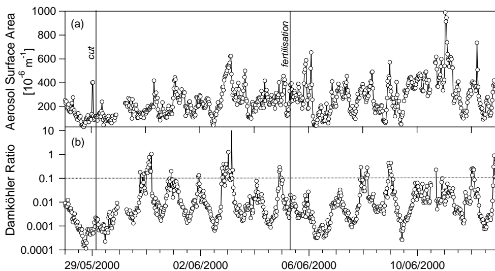
Fig. 6. Time-series of the aerosol surface area and the Damköhler ratio ( D_r = \tau_v / \tau_c ). The dashed line represents the critical value of D_r , above which chemistry is expected to alter the vertical gradients.
