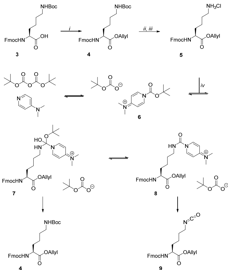
Scheme 1. Postulated mechanism by Knölker and co-workers to convert a free amine to the isocyanate applied to starting material 5 . 31 Reagents and conditions: ( i ) \text{Ag}_2\text{CO}_3 , allyl bromide, DMF, 0^\circ\text{C} to rt, 2.5 hrs, 95% ( ii ) \text{SnCl}_4 , DCM, EA, rt, 1 hr, 88% ( iii ) DMAP, MeCN, rt, 5 min. ( iv ) \text{Boc}_2\text{O} , DMAP, MeCN, rt, 10 min., 68% ( 3 ).
