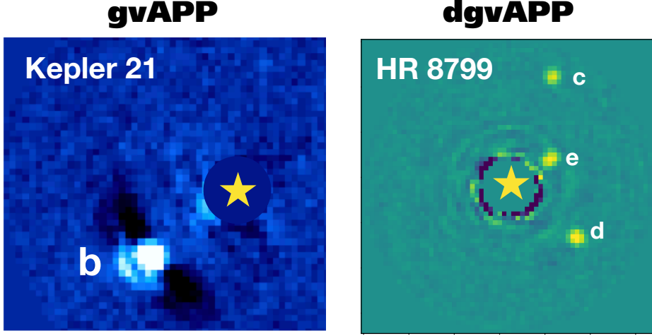
Figure 2.17: Detection of Kepler 21B using the gvAPP at LBT/LMIRcam ( \Delta m = 3.9 and the inner three HR 8799 planets ( \Delta m = \sim 10 ) using the dgvAPP at LMIRcam/ALES.
