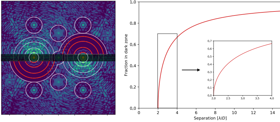
Figure 2.10: Planets rotating in the dark zone in pupil-stabilized mode are not always in the dark zone. Left : Fraction of a circle (white) that is in the dark zone (red). Right : The same fraction as function of separation for an inner working angle of 2\lambda/D .
