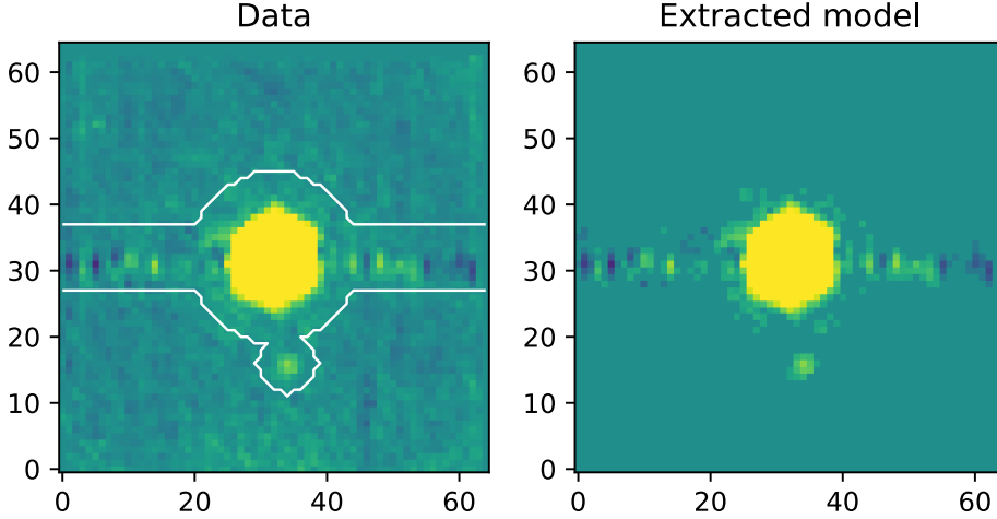
Figure 3.4: Left : Background-subtracted PSF at 3.55\ \mu\text{m} , using 10 PCA components of the 99 background frames. Residual structures indicate the presence of a ghost, some speckles, and a horizontal oscillating structure. Right : Same as left, but clipped at 2\sigma inside the area of a mask, indicated by the white lines left image.
