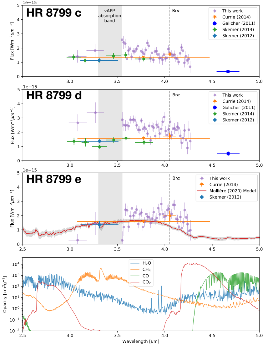
Figure 3.8: Spectra recovered with negative planet injection for HR 8799 cde, showing flux at 10 pc. We use the data 3.3\ \mu\text{m} magnitudes from Skemer et al. (2012), the different narrow-band magnitudes from Skemer et al. (2014), the broad L' -band and Br \alpha magnitudes from Currie et al. (2014), and the M-band magnitudes from (Galicher et al., 2011). In addition, we add the best-fit model for HR 8799 e from Mollière et al. (2020). The bottom panel shows the opacities of H 2 O, CH 4 , CO, and CO 2 in the same wavelength range, calculated with PetitRADTRANS for a temperature of 1200 K and a pressure of 1 bar. (Mollière et al., 2019).
