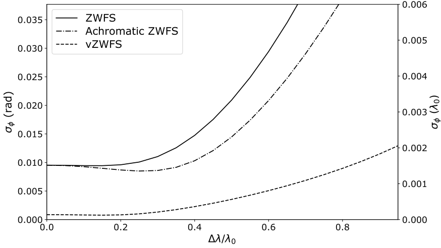
Figure 7.5: Residual wavefront aberrations as function of bandwidth for both the classical ZWFS and the vZWFS. The "achromatic ZWFS" uses the classical ZWFS reconstruction on one pupil of the vZWFS.
