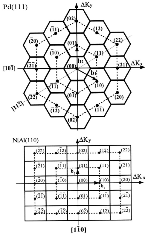
FIG. 2. Reciprocal space for the Pd(111) and NiAl(110) surfaces showing 2D Wigner–Seitz cells around each lattice point. Numbers within parentheses indicate the corresponding Miller indices. Dashed lines show diffraction orders. Numbers within brackets indicate the incidence directions considered in this work.
