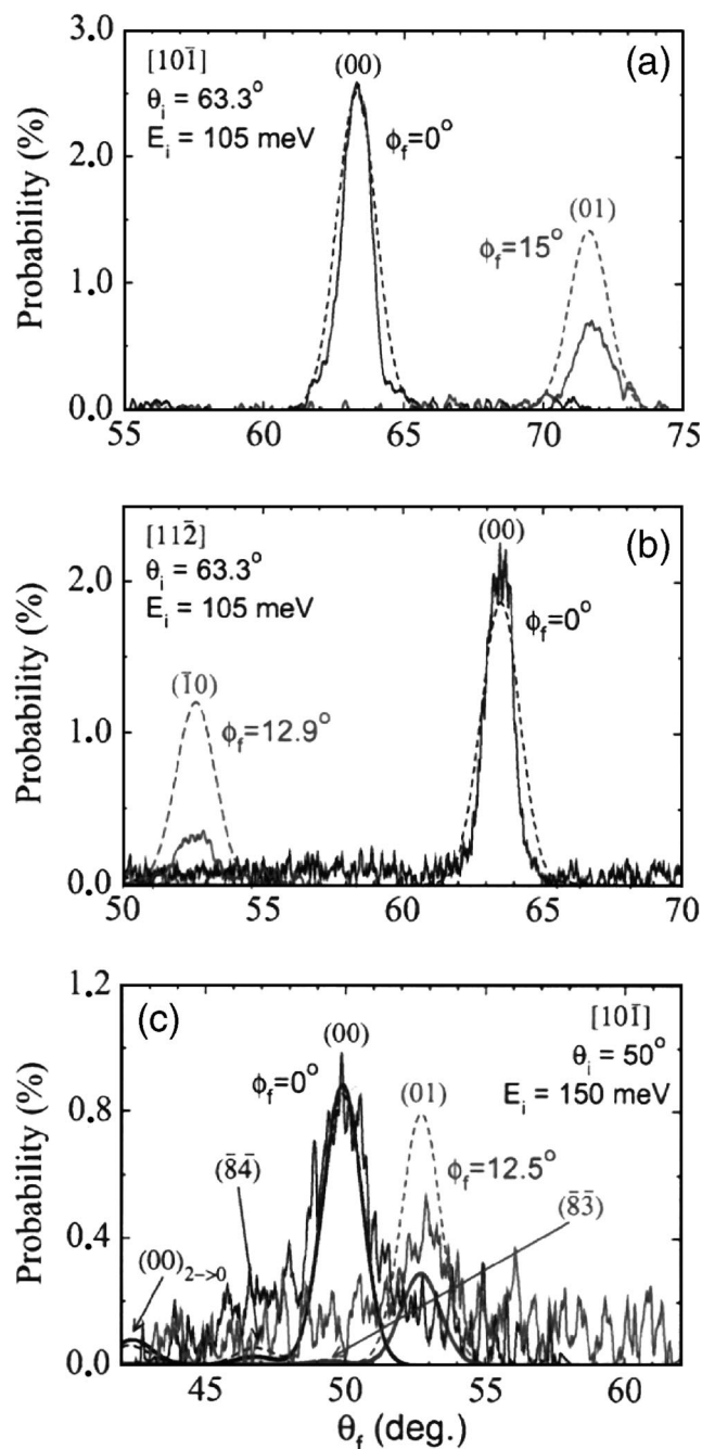
FIG. 5. (Color online) Diffraction spectra for \text{H}_2/\text{Pd}(111) at different incidence conditions. Black curves: in-plane diffraction. Green curves: out-of-plane diffraction. Full lines: experimental results (two upper panels, Ref. 31; lower panel, Ref. 58). Dashed lines: results of the classical diffraction method. Thick full lines: results of the quantum calculations. Theoretical peaks have been convoluted with a Gaussian function of width \sigma=0.7^\circ to account for the limited angular resolution of the experiment. Experimental and classical results have been normalized to the intensity of the specular peak obtained in the quantum calculations. Numbers within brackets indicate the incidence plane. The angle \phi_f is defined as in Fig. 4.
