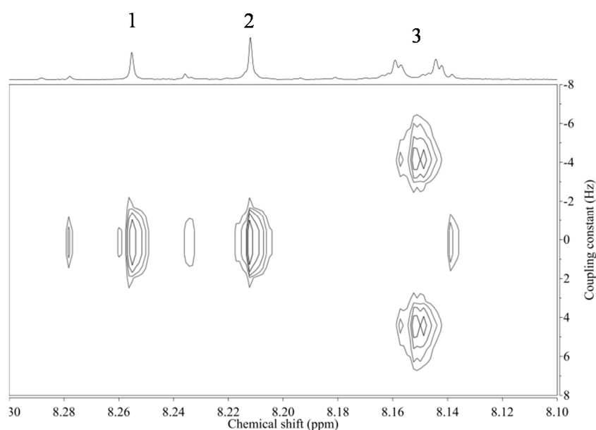
Figure 4. 1 H- 1 H-J-resolved spectrum of Astragalus membranaceus roots collected in the Shanxi province in China (No. of voucher specimen: 20131206-5) in CD 3 OD. 1: H-2 of formononetin-7- O -glucoside, 2: H-2 of calycosin-7- O -glucoside, 3: H-5 of formononetin-7- O -glucoside and calycosin-7- O -glucoside.
