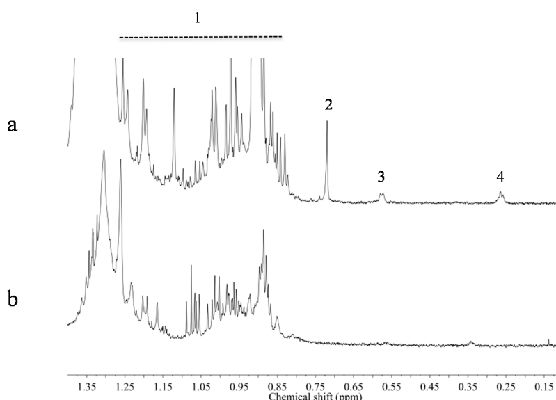
Figure 2. 1 H-NMR spectra of Astragalus membranaceus roots collected in Shanxi province in China (No. of voucher specimen: 20131206-2). (a) In CD 3 OD; (b) CD 3 OD-KH 2 PO 4 buffer in D 2 O (1:1, v/v), 1: methyl signals of astragaloside I, II, III, IV, isoleucine, leucine, and valine, 2: H-24 of astragaloside VIII and soyasaponin I, 3: H-19a of astragalosides, 4: H-19b of astragalosides.
