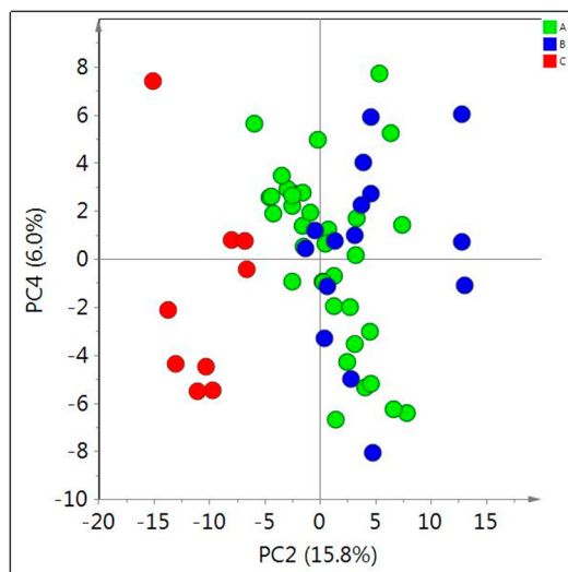
Figure 5. Score plot of principal component analysis (PCA, PC2/PC4) obtained from ^1\text{H} -NMR data of in \text{CD}_3\text{OD} extracts of 2–3 year old Astragalus membranaceus var. mongholicus (A); Asragalus membranaceus (B); and Hedysarum polybotrys (C).
