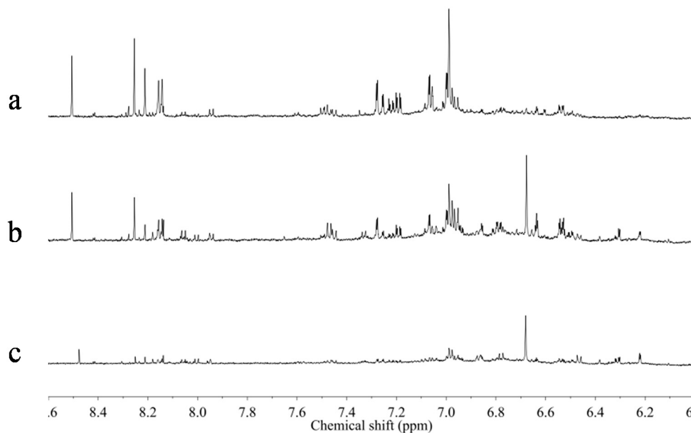
Figure 7. ^1\text{H} -NMR spectra ( \text{CD}_3\text{OD} ) of 30 (a), 20 (b), and 5 years (c) old Astragalus roots collected from Shanxi province in China.
