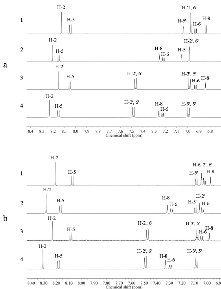
Figure 3. 1 H-NMR spectra of calycosin (1), calycosin-7- O -glucoside (2), formononetin (3), and formononetin- O -glucoside (ononin, 4). (a) In CD 3 OD; (b) CD 3 OD-KH 2 PO 4 buffer in D 2 O (1:1, v/v).
