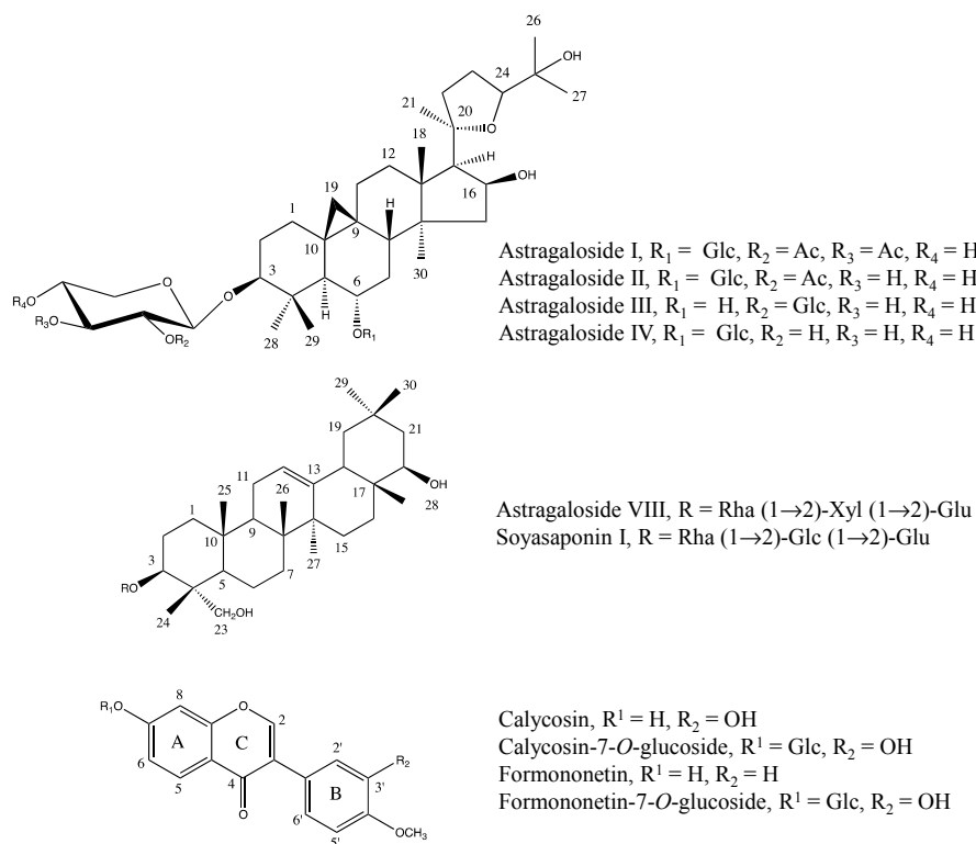
Figure 1. Chemical structures of typical saponins and flavonoids of Astragalus roots.
