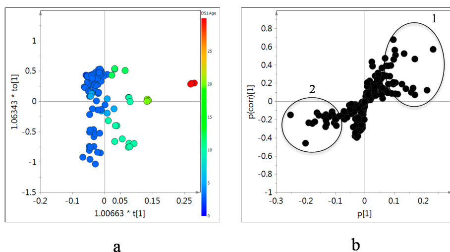
Figure 6. Score (a) and S-plot (b) of orthogonal partial least square (OPLS) modeling obtained from ^1\text{H} -NMR data of in \text{CD}_3\text{OD} extracts of Astragalus roots as X-data and age of each sample as Y-data. 1: H-2, H-5, H-6 and H-8 of isoflavonoids, H-1 and H-2' of sucrose, and H-3 of alanine, 2: H-2 and H-3 of asparagine and aspartic acid, \text{CH}_3 of choline, H-4 of GABA, and H-4 of proline.
