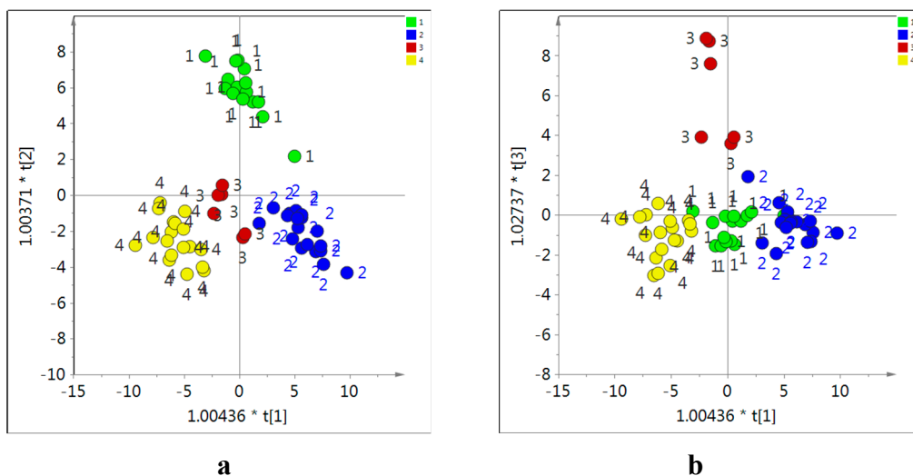
Figure 8. Score of orthogonal partial least square (OPLS) modeling obtained from ^1\text{H} -NMR data of in \text{CD}_3\text{OD} extracts of Astragalus roots as X-data and locations of each sample as Y-data using the combination of OPLS component 1 and 2 (a) and 1 and 3 (b). 1: Neimenggu, 2: Gansu, 3: Shanxi, 4: Shaanxi in China.
