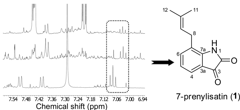
Figure 4. NMR-guided purification of 7-prenylisatin from Streptomyces sp. MBT28-91. Characteristic proton signals at \delta 7.03 (t, J = 7.2 Hz) that correlated to the high bioactivity are boxed (dashed box), which were used as tracking signals for chromatographic separation. Chemical shift divergence was due to the different deuterated solvents used (methanol- d_4 for top and middle rows and \text{CDCl}_3 for bottom row).
