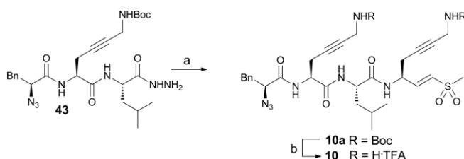
Scheme 3. Synthesis of compound 10 as example of an azide coupling followed by Boc removal. Reagents and conditions: a) 1) t BuONO, HCl, DMF; 2) H-Lys(4-yne)-VS, DiPEA; b) TFA, 79 % over two steps.
