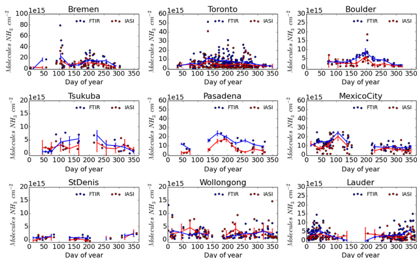
Figure 4. Time series of NH 3 for IASI and FTIR datasets with x_{\text{diff}} < 25 km and t_{\text{diff}} < 90 min (FTIR: blue and IASI: red). Scattered values are the observations for each day of year (multiple years of observations). The lines show the monthly mean total columns of the respective sets.
