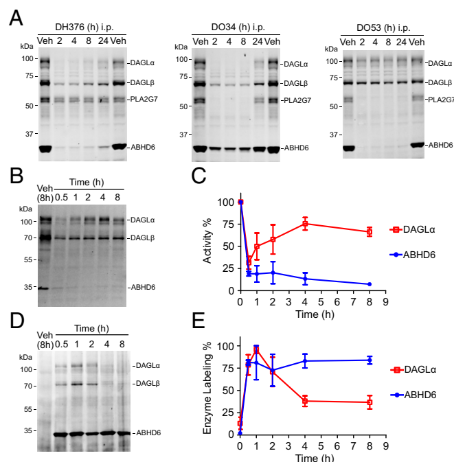
Fig. 3. Time-course analysis of DAGL \alpha inhibition and recovery. (A) Time course of inhibition of DAGL \alpha in brain tissue from mice treated with vehicle (Veh) or DH376, DO34, and DO53 (50 mg/kg, i.p. ) as determined by competitive ABPP using the DH379 probe (1 \mu M, 30 min). (B and C) Time course of inhibition of DAGL \alpha in brain tissue from mice treated with a low dose of DH376 (3 mg/kg, i.p. ) as determined by competitive ABPP using the DH379 probe (1 \mu M, 30 min). Gel data (B) and quantification of these data (C) relative to a vehicle-treated control group are shown for both DAGL \alpha and ABHD6, an off-target of DH376. Data represent average values \pm SEM; n = 3 mice per group. (D and E) Time course of direct labeling of DAGL \alpha in brain tissue from mice treated with DH376 (3 mg/kg, i.p. ) visualized by CuAAC to a Cy5 reporter group. Gel data (D) and quantification of these data (E) relative to a vehicle-treated control group are shown for both DAGL \alpha and ABHD6. Data represent average values \pm SEM; n = 3 mice per group.
