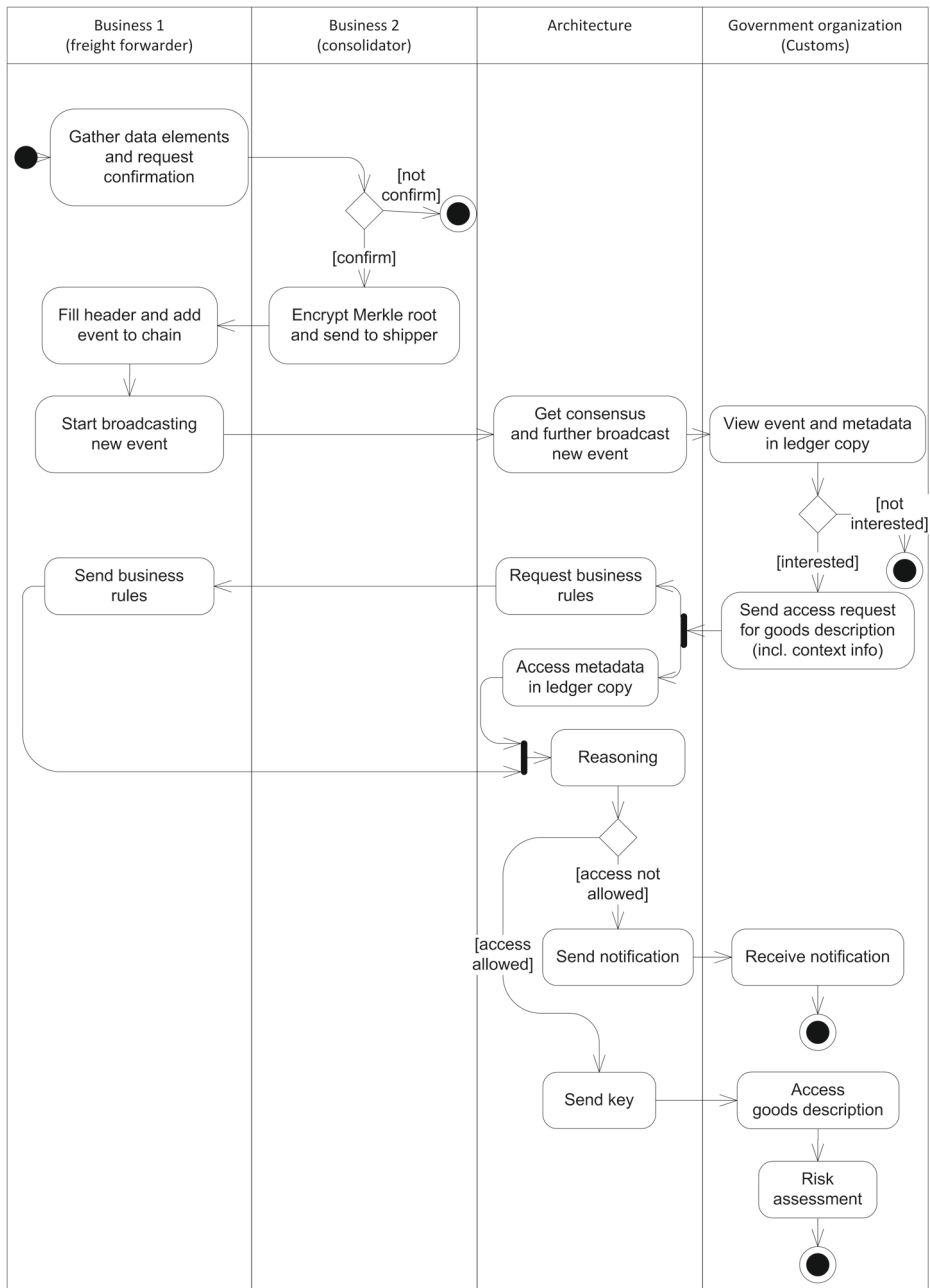
Fig. 4 UML activity diagram demonstration of typical user activity (Fowler and Scott 1999)
