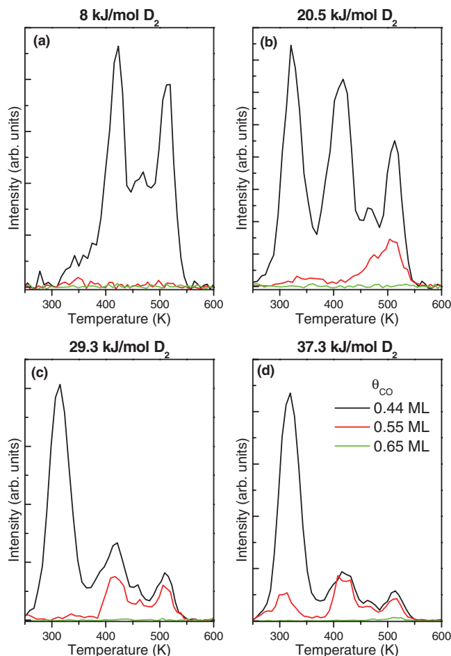
FIG. 2. D 2 TPD traces obtained after molecular beam dosing of D 2 with translational energies of (a) 8 kJ/mol, (b) 20.5 kJ/mol, (c) 29.3 kJ/mol, and (d) 37.3 kJ/mol on to Ru(0001) with \theta_{\text{CO}} = 0.44 ML (black), = 0.55 ML (red), and = 0.65 ML (green). Note that the intensity scales on the individual panels differ from each other.
