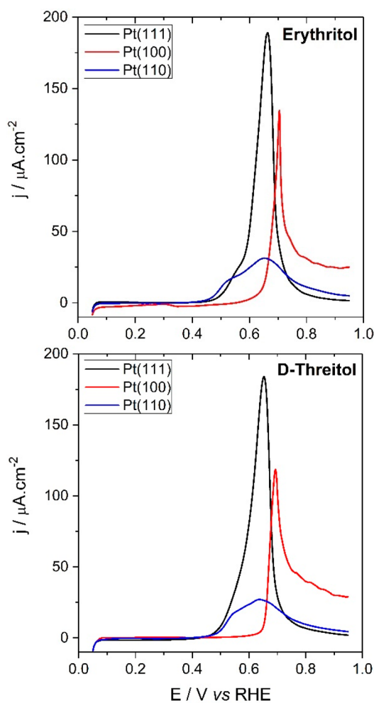
Figure 3. Positive-going sweep of the 1st cycle of the voltammetric response for the erythritol and D-threitol oxidation in 0.1 mol L -1 \text{HClO}_4 + 5 mmol L -1 polyol on Pt(111) and Pt(100). Sweep rate of 1 mV s -1 .
