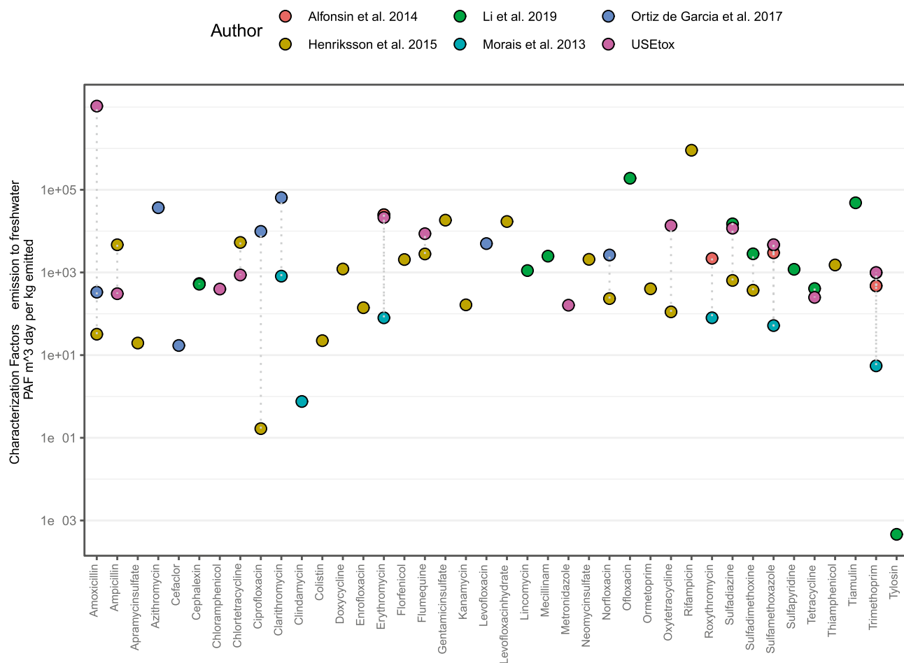
Fig. 1 Available CFs for AB emissions to freshwater calculated using USEtox, FETP=freshwater ecotoxicity potential. Units are presented in PAF m 3 day kg -1 emitted
