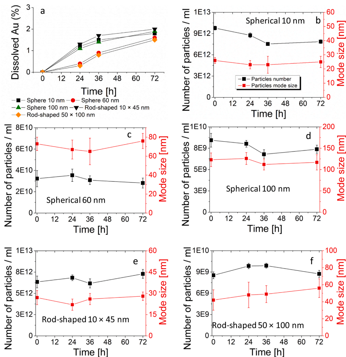
Fig. 1. a) The percentage of dissolved Au in the exposure media over 72 h incubation time. b-f) The particle number of Au-NP (black line) and the measured mode size of the size distribution (red line) over the duration of the exposure in the exposure media without algae cells. (For interpretation of the references to color in this figure legend, the reader is referred to the web version of this article.)
