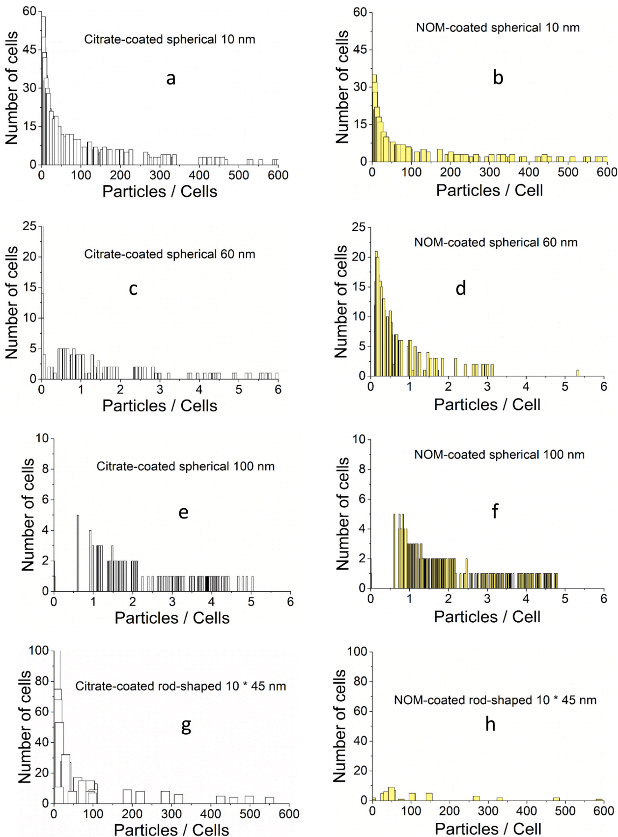
Fig. 3. The number of Au-NP accumulated on the surface of each algal cell within a given population as a function of particle size and shape and in the presence and absence of NOM. The number distribution of the spherical 10 nm Au-NPs (a-b), the spherical 60 nm Au-NPs (c-d), the spherical 100 nm Au-NPs (e-f), and the rod-shaped 10 × 45 nm Au-NPs (g-h).
