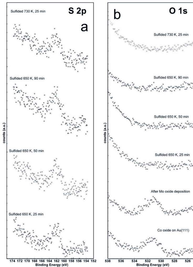
Figure S5:a,b) XPS spectra of S 2p and O 1s regions respectively at various stages of the oxide precursor synthesis and subsequent sulfidation.
