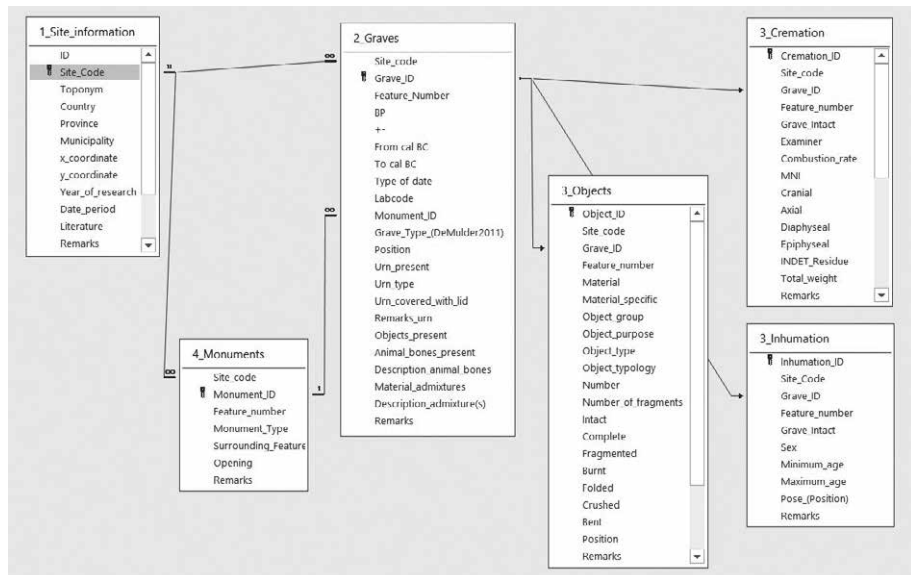
Fig. 3.8: Printsreen of the database structure.
