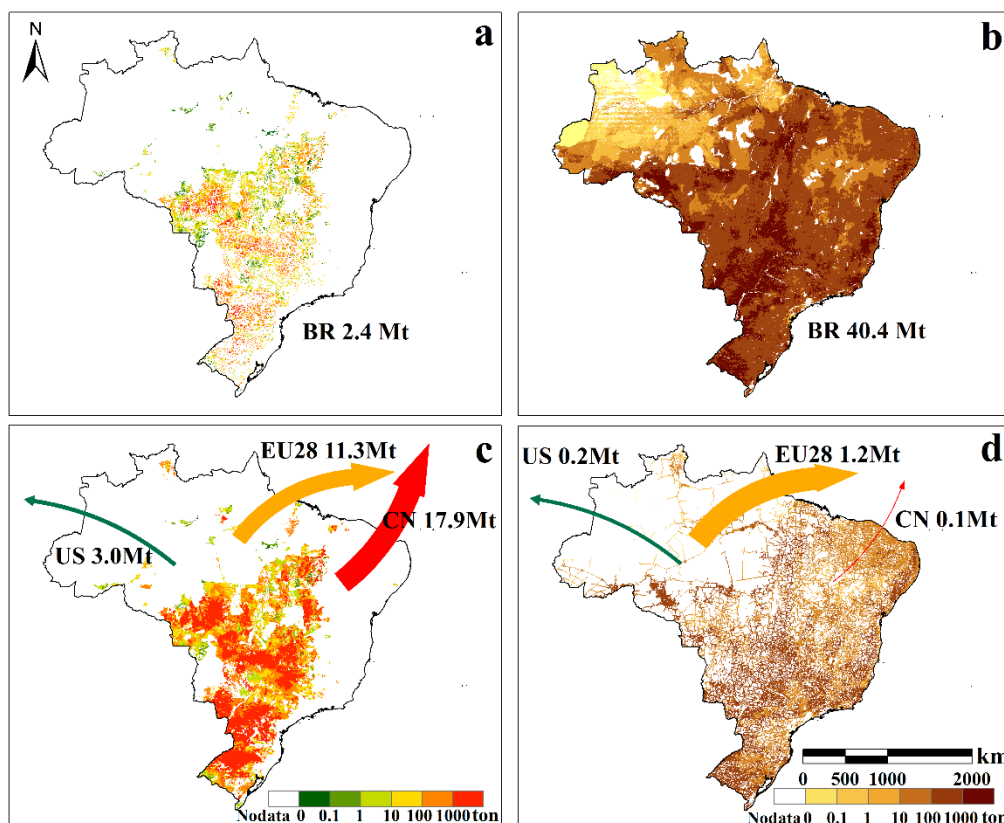
Figure 3.2 Brazilian soybeans and beef for domestic consumption (a, b) and consumption in foreign countries (c, d).
