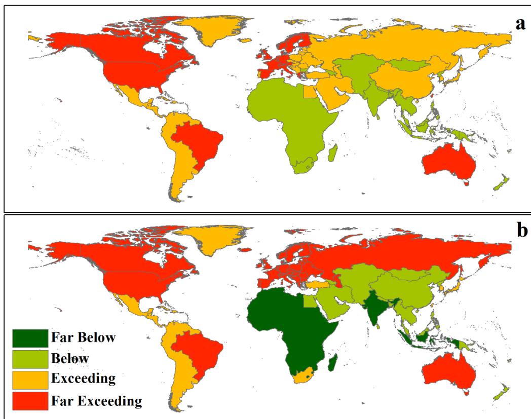
Figure 3.4 Total primary crop (a) and livestock (b) consumption per-capita in comparison with the tentative target of 0.9 and 0.12 ton per-capita in 2006, respectively.
