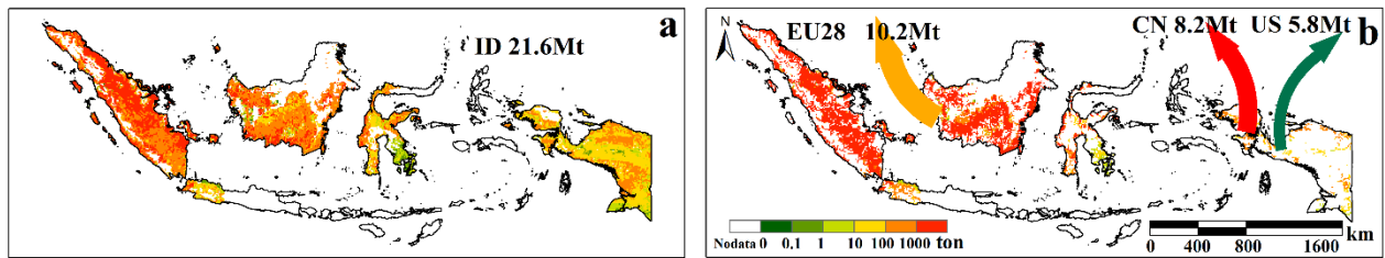
Figure 3.3 Indonesian palm oil for domestic (a) and foreign consumption (b).
