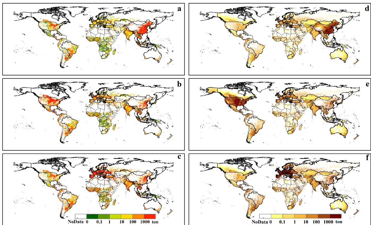
Figure 3.1 Spatial distribution of the primary crop hotspots driven by consumption of China (a), the US (b), and the EU28 (c), and the livestock hotspots driven by consumption of China (d), the US (e) and the EU28 (f).
