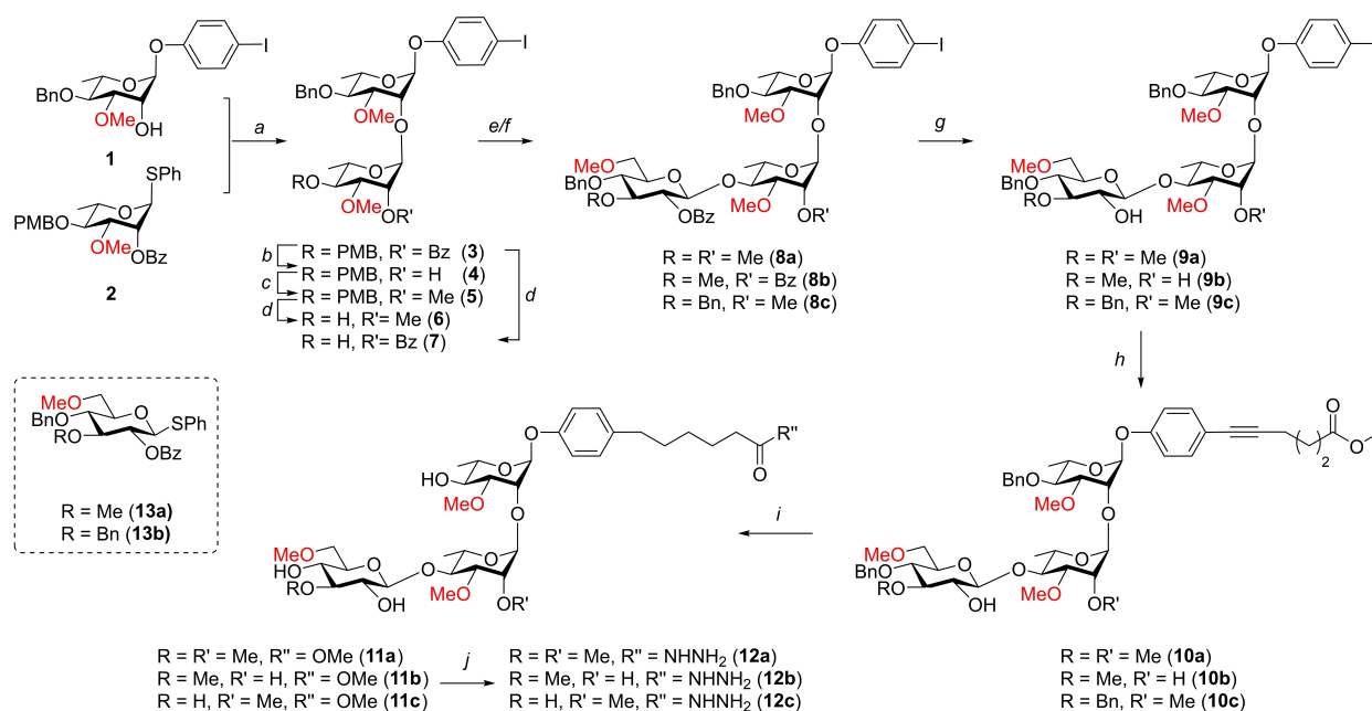
Scheme 1. a) \text{Ph}_2\text{SO} , \text{Tf}_2\text{O} , TTBP, \text{CH}_2\text{Cl}_2 , -60^\circ\text{C} , 66%; b) Na, MeOH/THF, 97%; c) NaH, MeI, DMF, 95%; d) HCl/HFIP, HFIP/ \text{CH}_2\text{Cl}_2 , 93% (6), 100% (7); e) Donor 13a, \text{Ph}_2\text{SO} , \text{Tf}_2\text{O} , TTBP, \text{CH}_2\text{Cl}_2 , -60^\circ\text{C} , 93% (8a), 88% (8b); f) Donor 13b, \text{Ph}_2\text{SO} , \text{Tf}_2\text{O} , TTBP, \text{CH}_2\text{Cl}_2 , -60^\circ\text{C} , 100% (8c); g) Na, MeOH/THF, 99% (9a), 84% (9b), 97% (9c); h) Methyl hex-5-ynoate, \text{Pd}(\text{PPh}_3)_2\text{Cl}_2 , \text{PPh}_3 , CuI, \text{Et}_3\text{N} , 99% (10a), 77% (10b), 82% (10c); i) \text{Pd/C} , \text{H}_2 , THF/MeOH, 100% (11a), 82% (11b), 90% (11c); j) \text{N}_2\text{H}_4\cdot\text{H}_2\text{O} , EtOH, 89% (12a), 100% (12b), 84% (12c).
