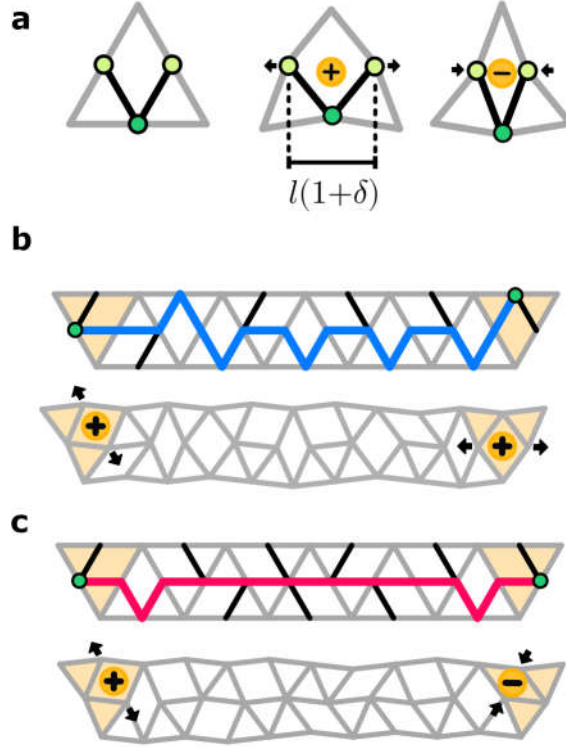
Fig. 3.12.: Understanding network mechanics with path parity. a , A single building block's floppy mode is actuated by displacing its majority edge-nodes (light green circles) to a positive or negative block spin (yellow markers), quantified by the block strain \delta . b , How connected building blocks deform depends on the parity of their connecting path (section 2.3.1) Top: two blocks (yellow triangles) are connected by a ferromagnetic path (blue line). Bottom: the blocks' spins have the same sign (yellow markers) under actuation of the strip's floppy mode. c , Alternatively, two blocks are connected by an antiferromagnetic path (red line). The blocks' spins are opposite when the floppy mode is activated.
