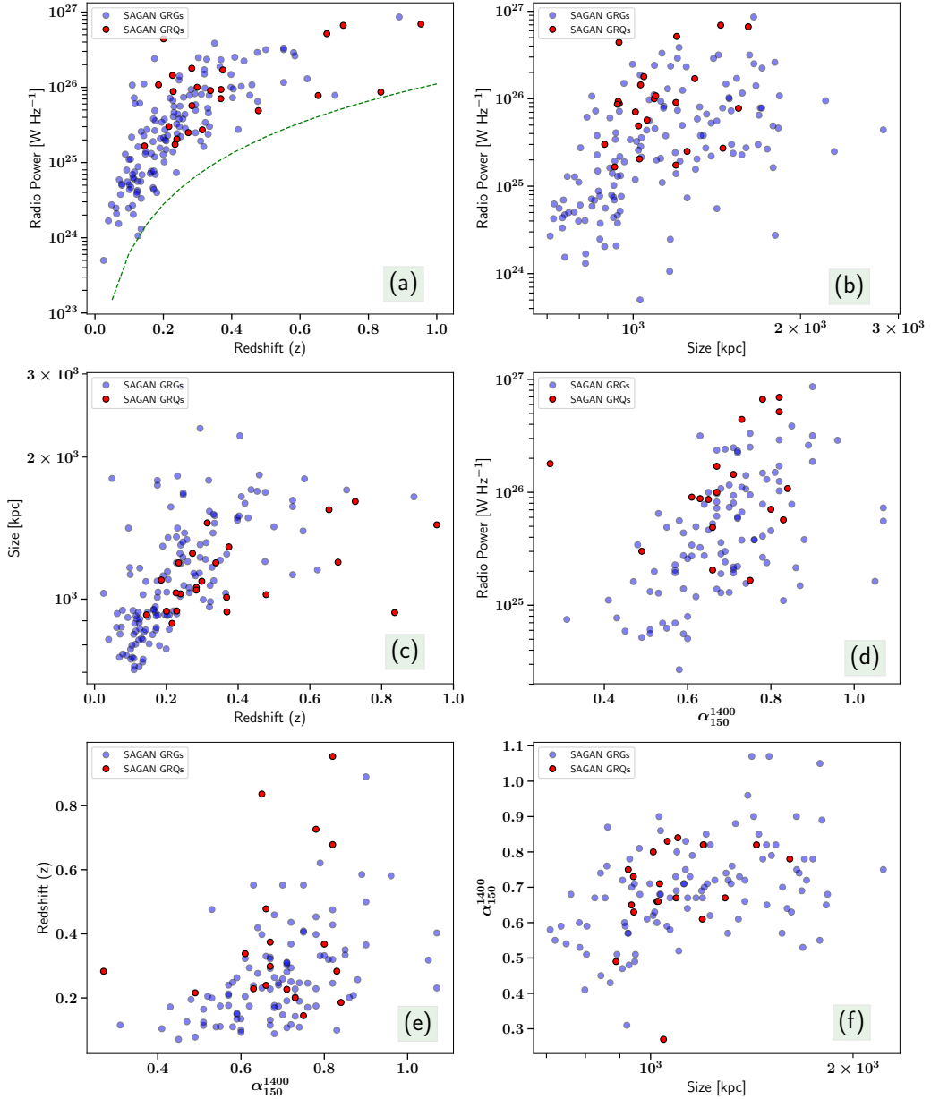
Figure 4.4: Correlations of radio power [ \text{W Hz}^{-1} ] at 1400 MHz, size [kpc], redshift, and spectral index for GRGs and GRQs. Red circles indicate GRQs, and blue circles indicate GRGs. The dashed green line in panel (a) represents the minimum radio luminosity corresponding to a flux density \sim 24\text{mJy} of source SAGANJ090640.80+142522.97 at different redshifts, assuming a spectral index of 0.75.
