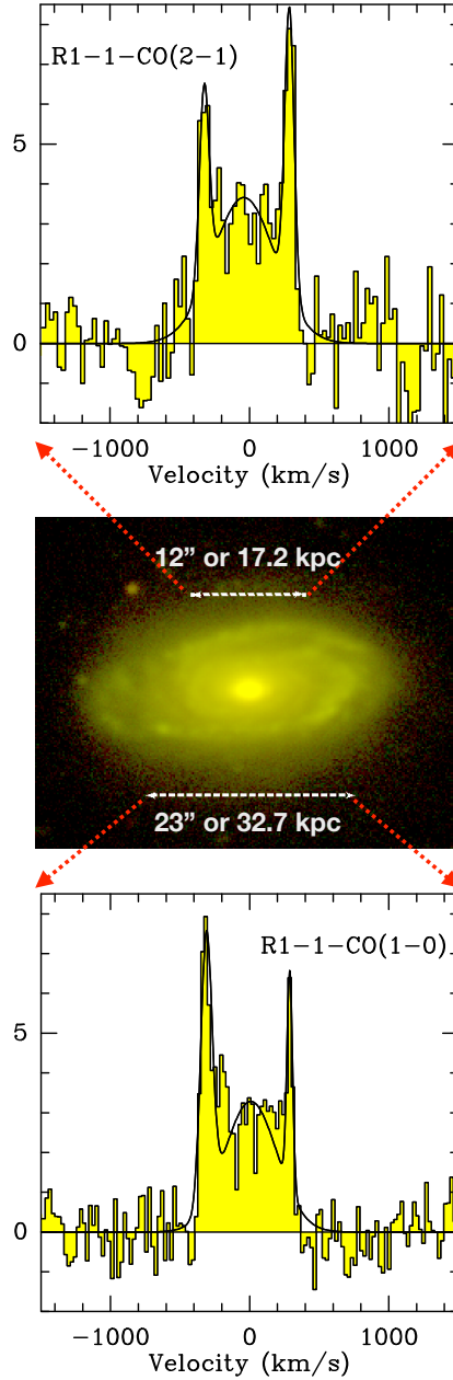
Figure 5.3: Two spectra obtained towards R1-1 or GRG-J2345–0449 in CO(1-0) (bottom) and CO(2-1) (top). The vertical scale is T_{mb} in mK. The middle optical image of the host spiral galaxy of J2345–0449 is obtained by combining G- and R-band data of MegaCam on the CFHT. The G and R-band data belong to the first-generation filters on the MegaCam. The scale on the image represents the beam of the IRAM observations at the respective frequencies.
