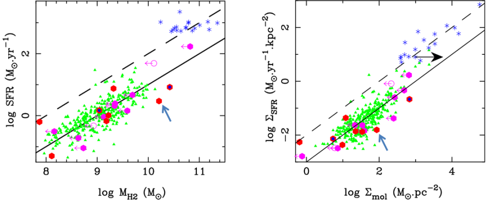
Figure 5.8: Star formation rate as a function of the molecular content for our targets compared to normal galaxies and starbursts at comparable redshifts. The global SFR- M_{\text{mol}} diagram is shown at the left, and the surface densities of the same quantities, representing the unresolved Kennicutt-Schmidt relation (Kennicutt 1998), are shown at the right. The straight lines are power laws of slope 1. The full line corresponds to a depletion time of 1 Gyr, and the dashed line to 100 Myr. Symbols are the same as in Figure 5.7; upper limits of our targets are shown in pink, and tentative detections as a blue hexagon inside the red one. The blue arrow points to the location of R1-1 (GRG-J2345-0449) in the respective plots.
