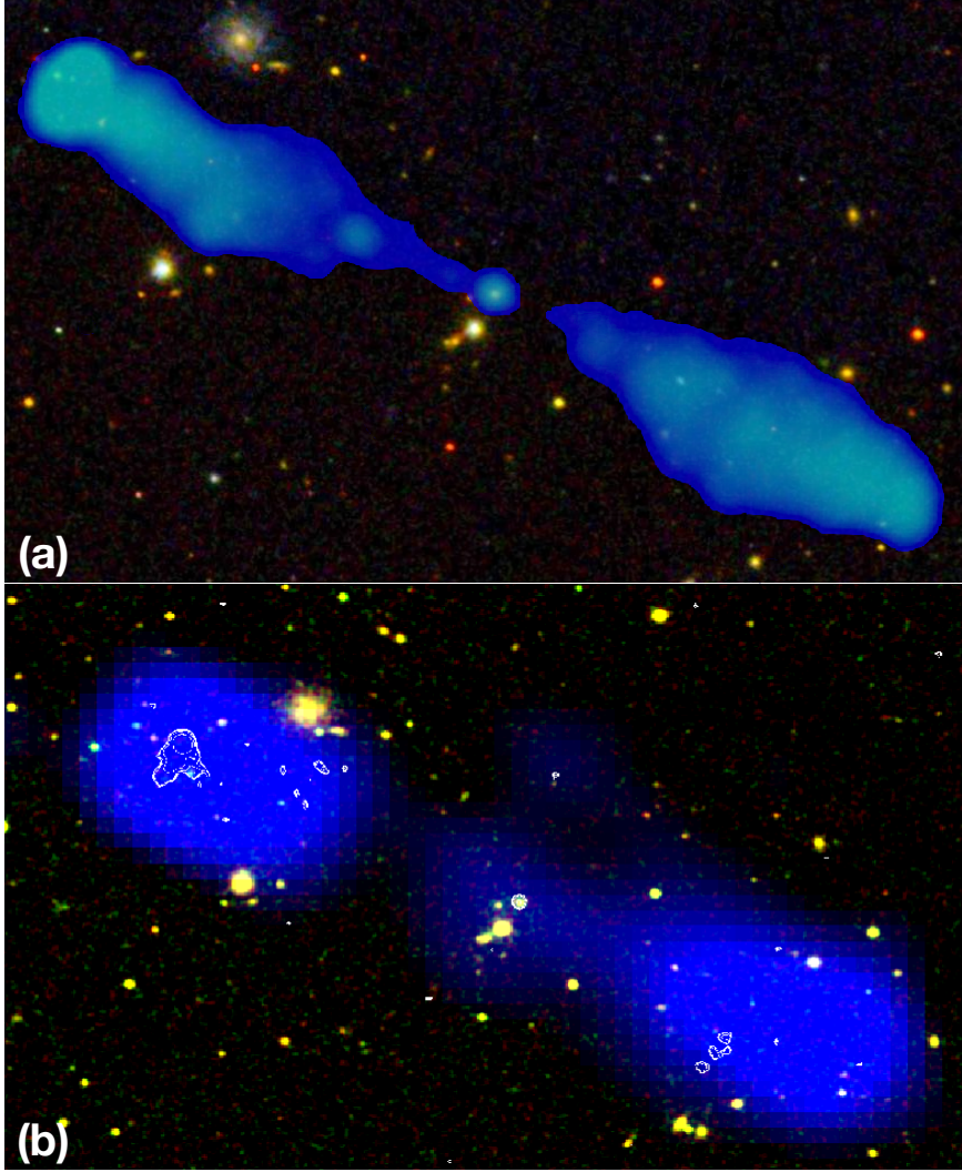
Figure 3.1: (a) A colour composite image of 1.86 Mpc long GRG J105817.90+514017.70 made using LoTSS-DR1 144 MHz radio and optical SDSS image. (b) A colour composite image of the same object with optical and radio overlay, where blue represents 1400 MHz NVSS image with 45'' resolution and white contours from 1400 MHz FIRST survey having 5'' resolution superimposed on optical SDSS image. The LoTSS 144 MHz 6'' resolution image shown in top panel clearly resolves the core and jet and also highlights the diffuse parts of the lobes, which is missed by the FIRST and unresolved in NVSS.
