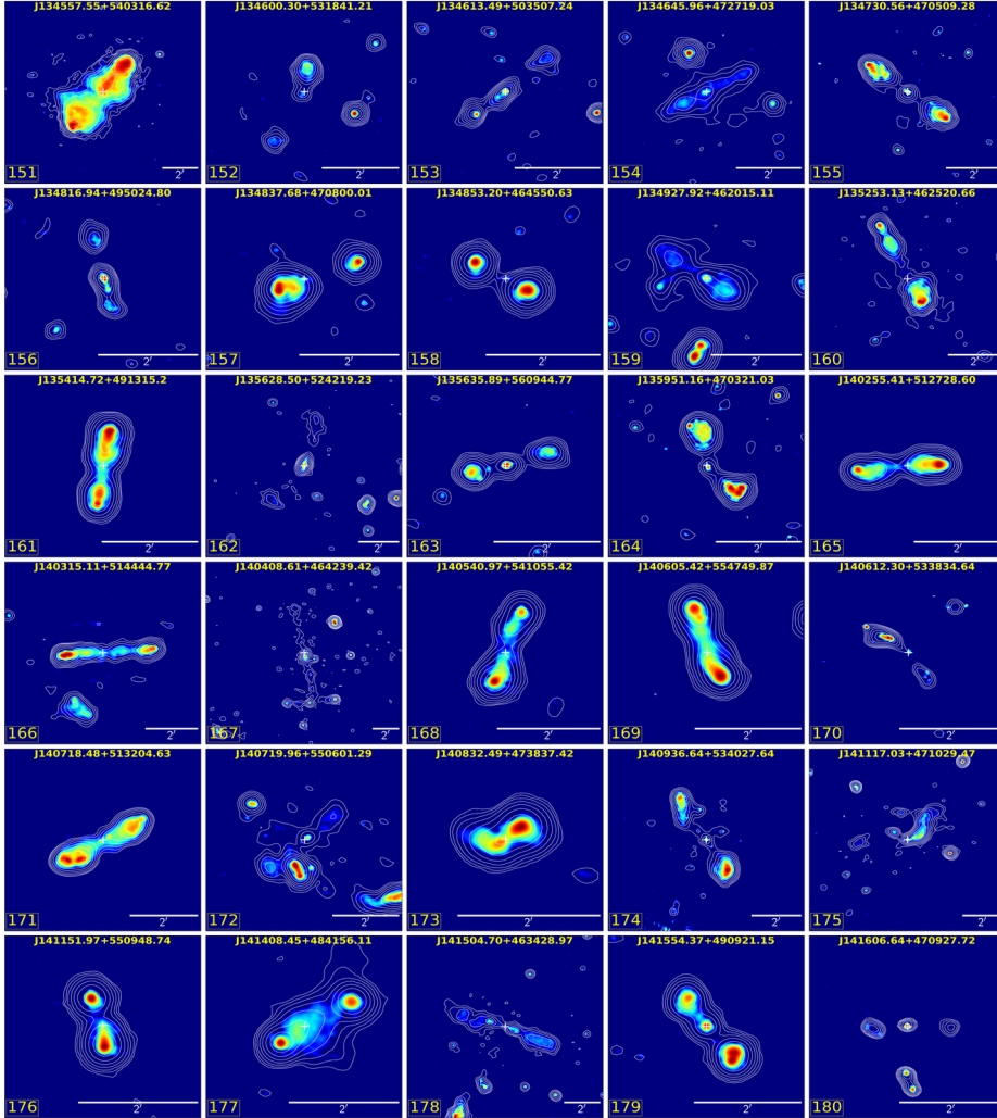
Figure 3.20: LoTSS high resolution ( \sim 6'' ) images 151-180 with LoTSS low resolution ( \sim 20'' ) contours overlaid. The cross '+' marker indicates the location of the host galaxy. The radio contours are drawn with 8 levels which are chosen by equally (log scale) dividing the data value range above \sim 3\sigma , where \sigma is the local RMS of the map.
