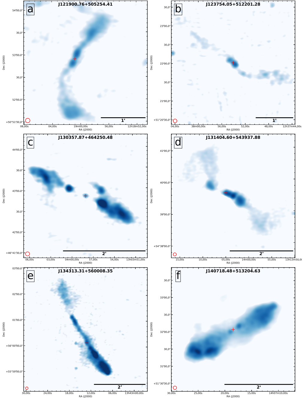
Figure 3.13: DDRGs postage-1 (7-12 DDRGs) made using LoTSS DR1 144 MHz radio image with 6'' \times 6'' resolution in inverted blue colour scale. Refer to Sect. 3.4.2 for more details.
