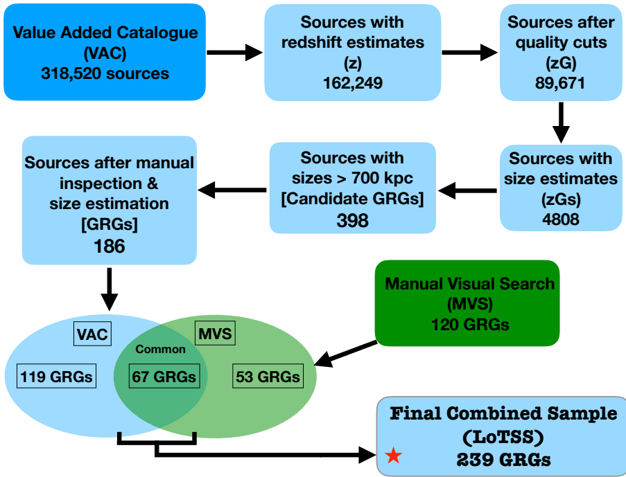
Figure 3.2: The above figure shows schematics for finding GRGs from LoTSS DR1 using VAC and MVS in steps. More details are presented in Sect. 3.2.
