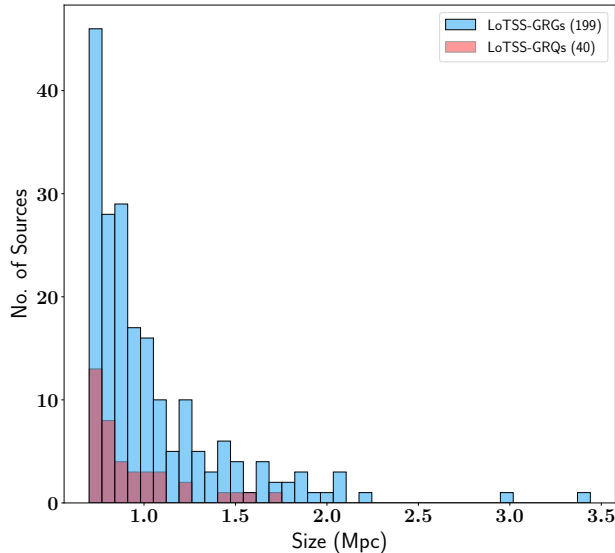
Figure 3.3: Histogram for sizes of GRGs and GRQs from the LoTSS sample.
