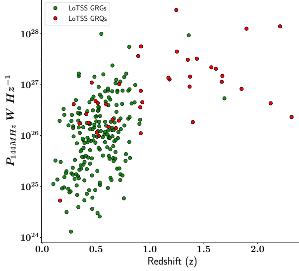
Figure 3.4: Radio power and redshift distribution for GRGs and GRQs from LoTSS. The two galaxies marked in green colour with z \geq 1 are quasar candidates as explained in Sec. 3.3.4.
