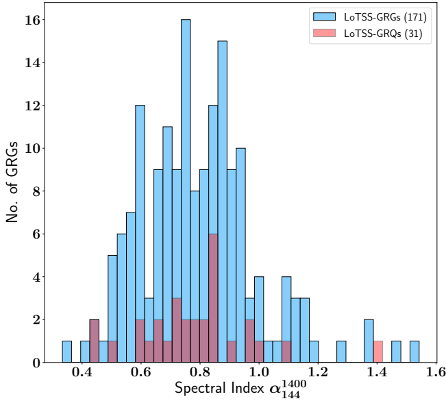
Figure 3.6: Histogram of Spectral index ( \alpha_{144}^{1400} ) of GRGs and GRQs in LoTSS DR1 sample made using LoTSS and NVSS.
