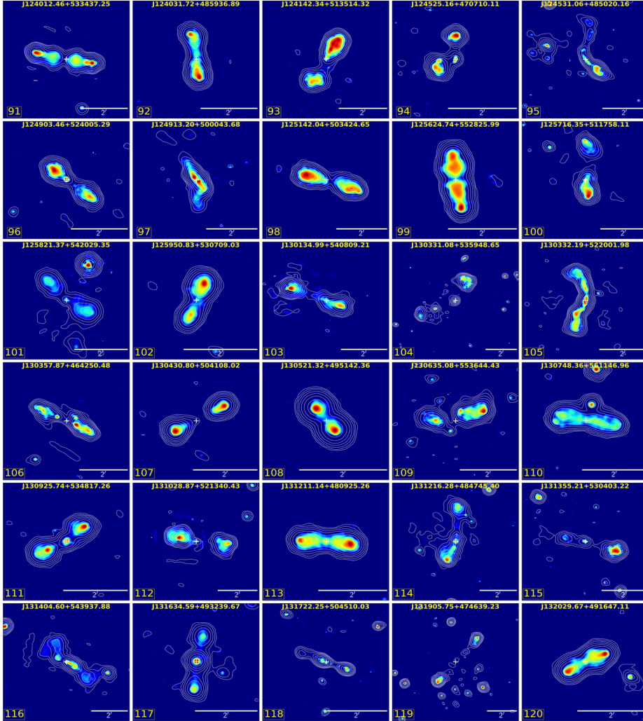
Figure 3.18: LoTSS high resolution ( \sim 6'' ) images 91-120 with LoTSS low resolution ( \sim 20'' ) contours overlaid. The cross '+' marker indicates the location of the host galaxy. The radio contours are drawn with 8 levels which are chosen by equally (log scale) dividing the data value range above \sim 3\sigma , where \sigma is the local RMS of the map.
