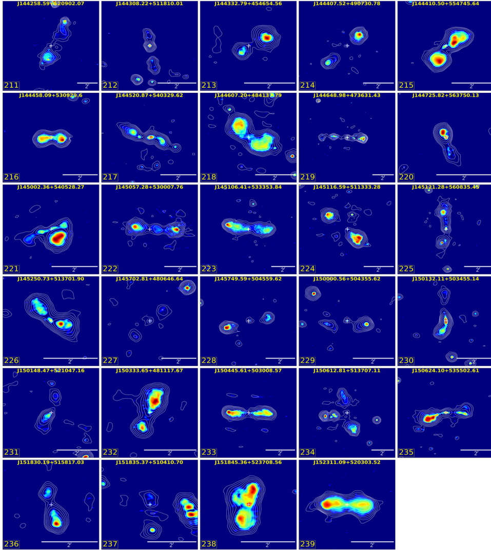
Figure 3.22: LoTSS high resolution ( \sim 6'' ) images 211-239 with LoTSS low resolution ( \sim 20'' ) contours overlaid. The cross '+' marker indicates the location of the host galaxy. The radio contours are drawn with 8 levels which are chosen by equally (log scale) dividing the data value range above \sim 3\sigma , where \sigma is the local RMS of the map.
