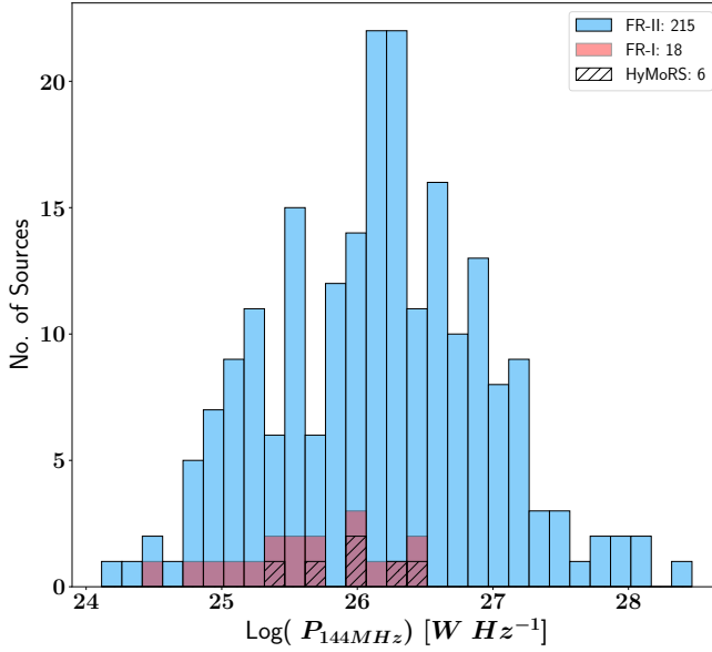
Figure 3.9: Radio power (144 MHz) distribution of FR-I, FR-II and HyMoRS sources in LoTSS DR1 sample of giants.
