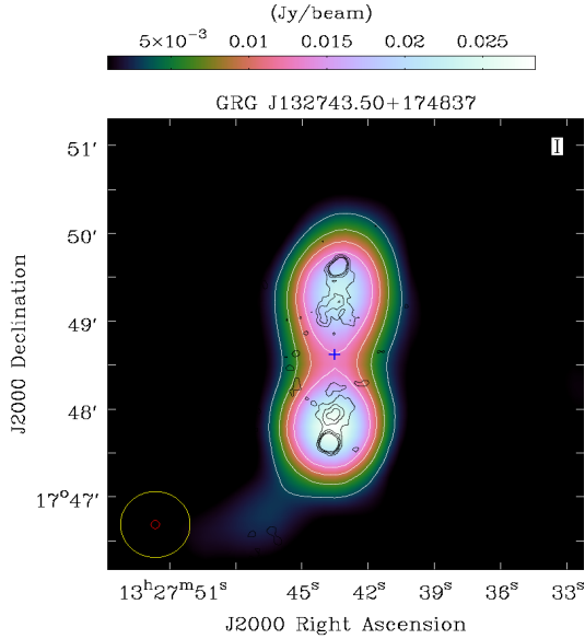
(k) GRG11 (Linear size = 1.33 Mpc)
