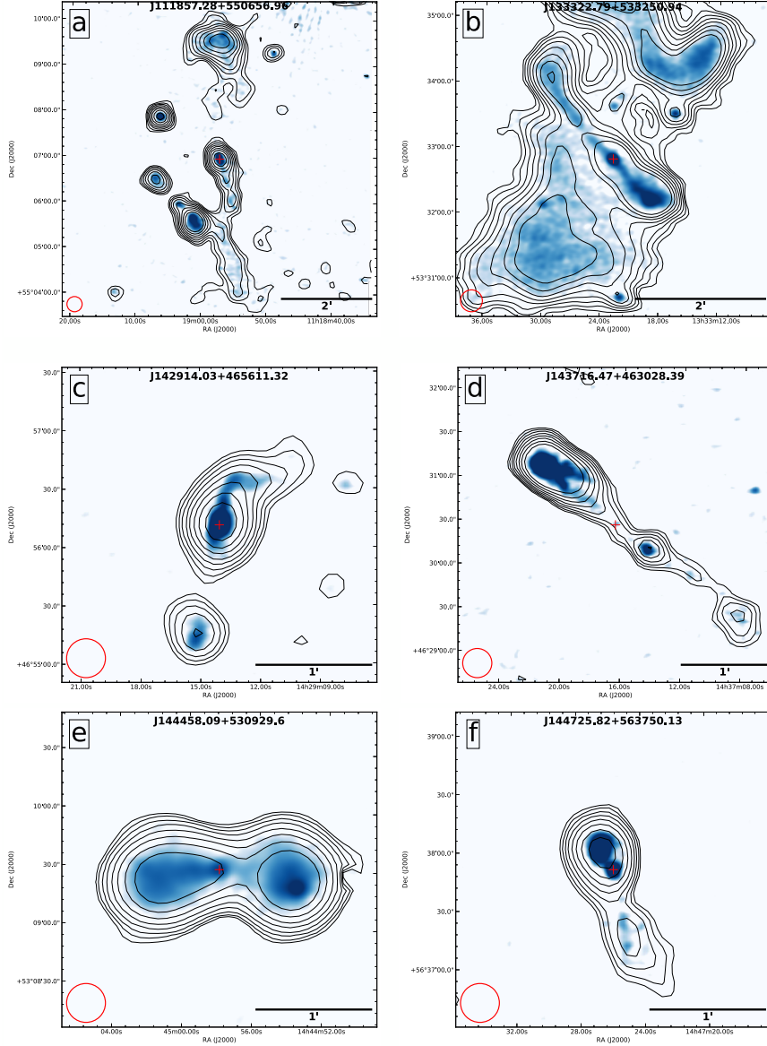
Figure 3.11: LoTSS DR1 ( 6'' \times 6'' ) maps of 6 HyMoRS in inverted blue colour scale with ( 20'' \times 20'' ) black contours (eight equally spaced relative contour levels starting from three times \sigma , where \sigma denotes the local RMS noise). The circles at bottom left corner represents the beam sizes of low resolution radio maps of LoTSS DR1. The red colour marker '+' indicates the location of the host galaxy.
