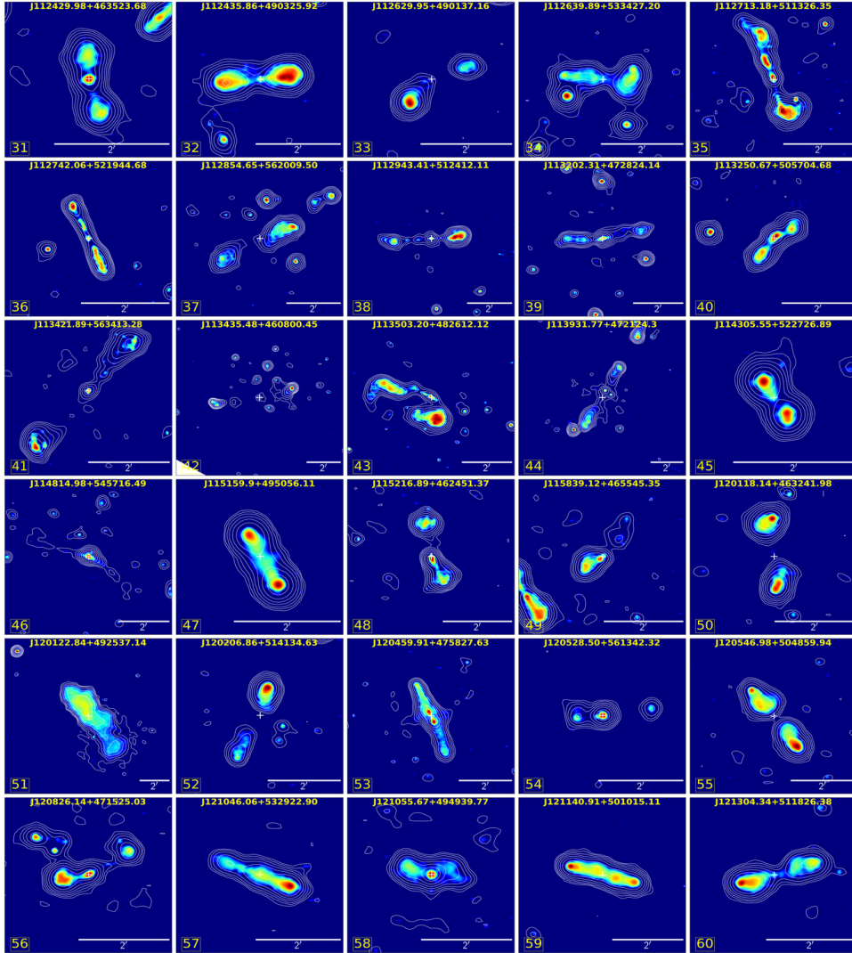
Figure 3.16: LoTSS high resolution ( \sim 6'' ) images 31-60 with LoTSS low resolution ( \sim 20'' ) contours overlaid. The cross '+' marker indicates the location of the host galaxy. The radio contours are drawn with 8 levels which are chosen by equally (log scale) dividing the data value range above \sim 3\sigma , where \sigma is the local RMS of the map.
