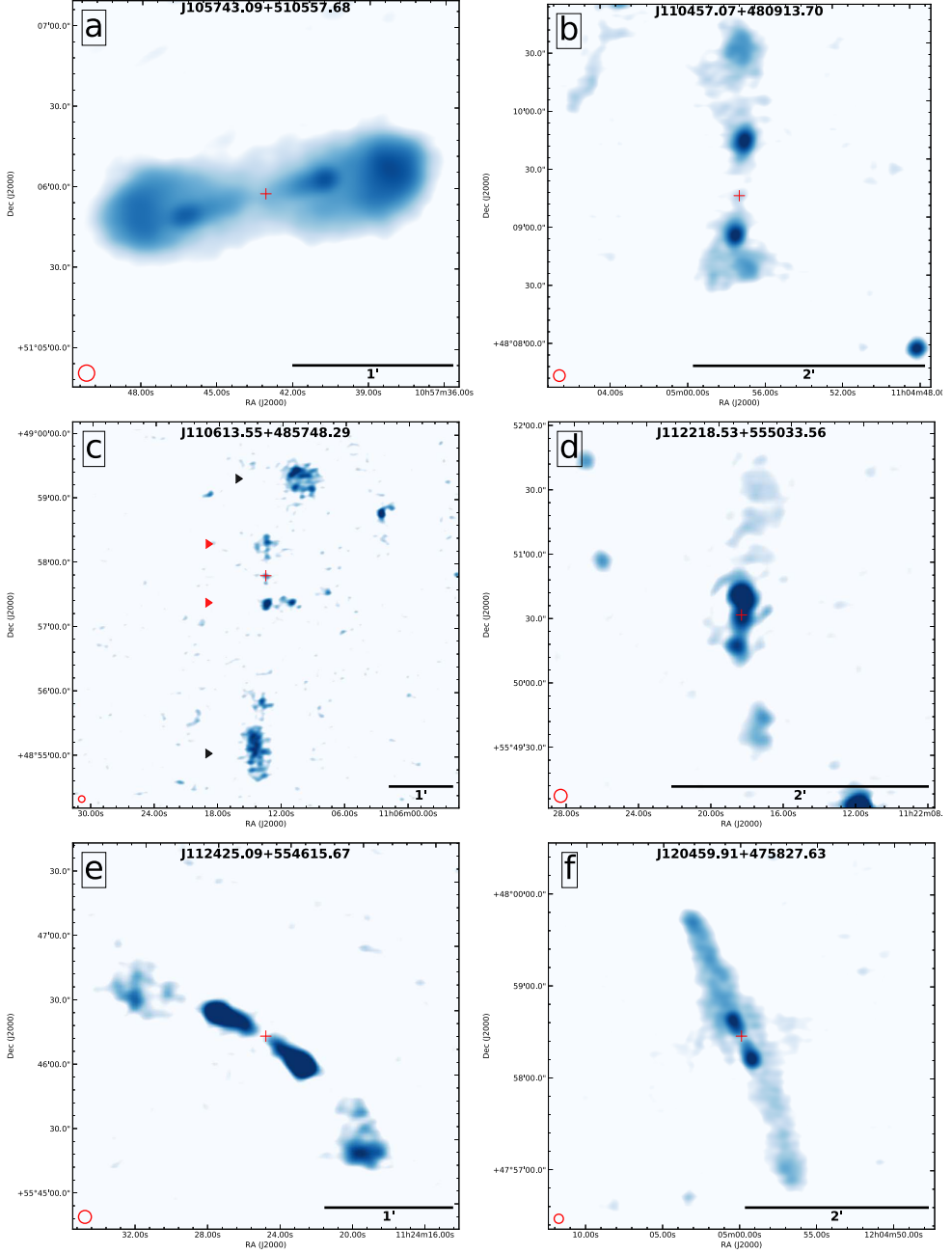
Figure 3.12: DDRGs postage-1 (1-6 DDRGs) made using LoTSS DR1 144 MHz radio image with 6'' \times 6'' resolution in inverted blue colour scale. Refer to Sect. 3.4.2 for more details. The circle at bottom left corner represents the beam size. The red colour marker ‘+’ indicates the location of the host galaxy. In source J110613.55+485748.29 (sub-image c) the two red markers indicate the inner pair of the DDRG and the black markers indicate the out pair of the DDRG.
