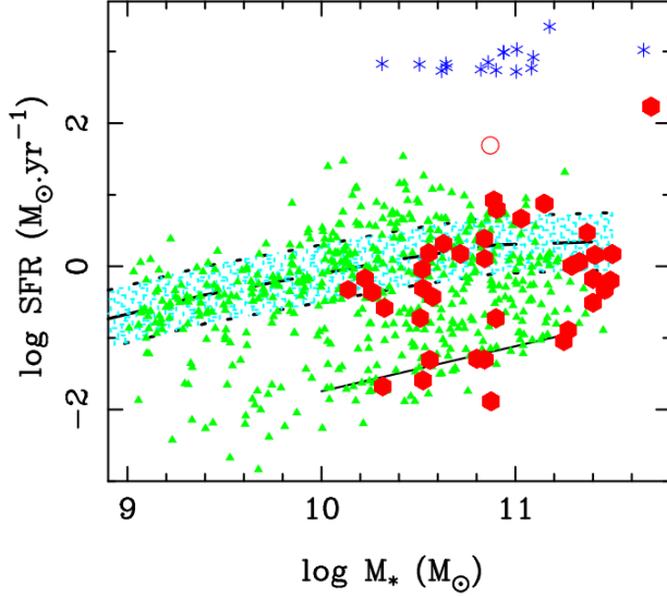
Figure 5.7: Location of our targets (red hexagons) in the SFR- M_{\text{star}} diagram. They are compared with the xCOLDBASS sample of 532 galaxies with local redshift 0.01 < z < 0.05 from Saintonge et al. (2017) (green triangles), and with the starburst galaxies (blue stars) in the comparable range 0.2 < z < 0.6 ( Combes et al. 2011 ). The SDSS main sequence is shown with the cyan-shaded region, and delimited by dashed lines (at \pm 0.4 dex), and the red sequence by a full line. Open red circles belong to non-GRGs observed by us.
