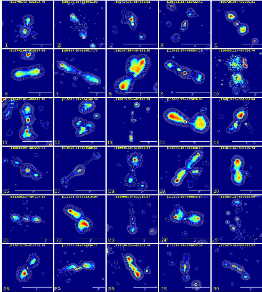
Figure 3.15: LoTSS high resolution ( \sim 6'' ) images 1-30 with LoTSS low resolution ( \sim 20'' ) contours overlaid. The cross '+' marker indicates the location of the host galaxy. The radio contours are drawn with 8 levels which are chosen by equally (log scale) dividing the data value range above \sim 3\sigma , where \sigma is the local RMS of the map.
