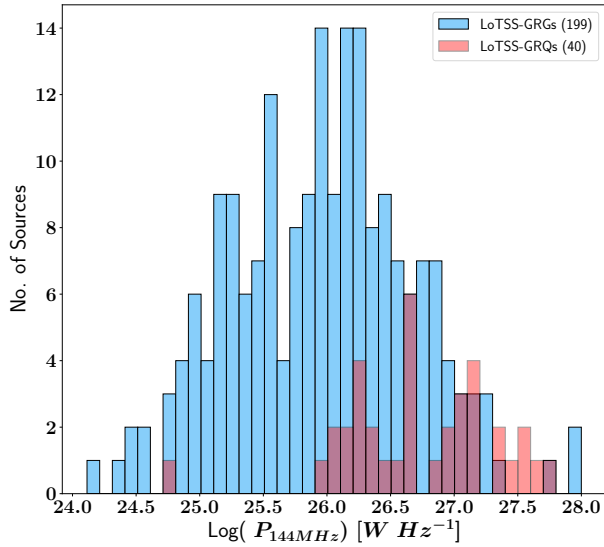
Figure 3.5: Histogram of radio power at 144 MHz of GRGs and GRQs.
