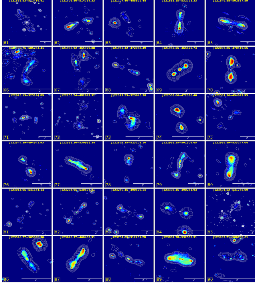
Figure 3.17: LoTSS high resolution ( \sim 6'' ) images 61-90 with LoTSS low resolution ( \sim 20'' ) contours overlaid. The cross '+' marker indicates the location of the host galaxy. The radio contours are drawn with 8 levels which are chosen by equally (log scale) dividing the data value range above \sim 3\sigma , where \sigma is the local RMS of the map.
