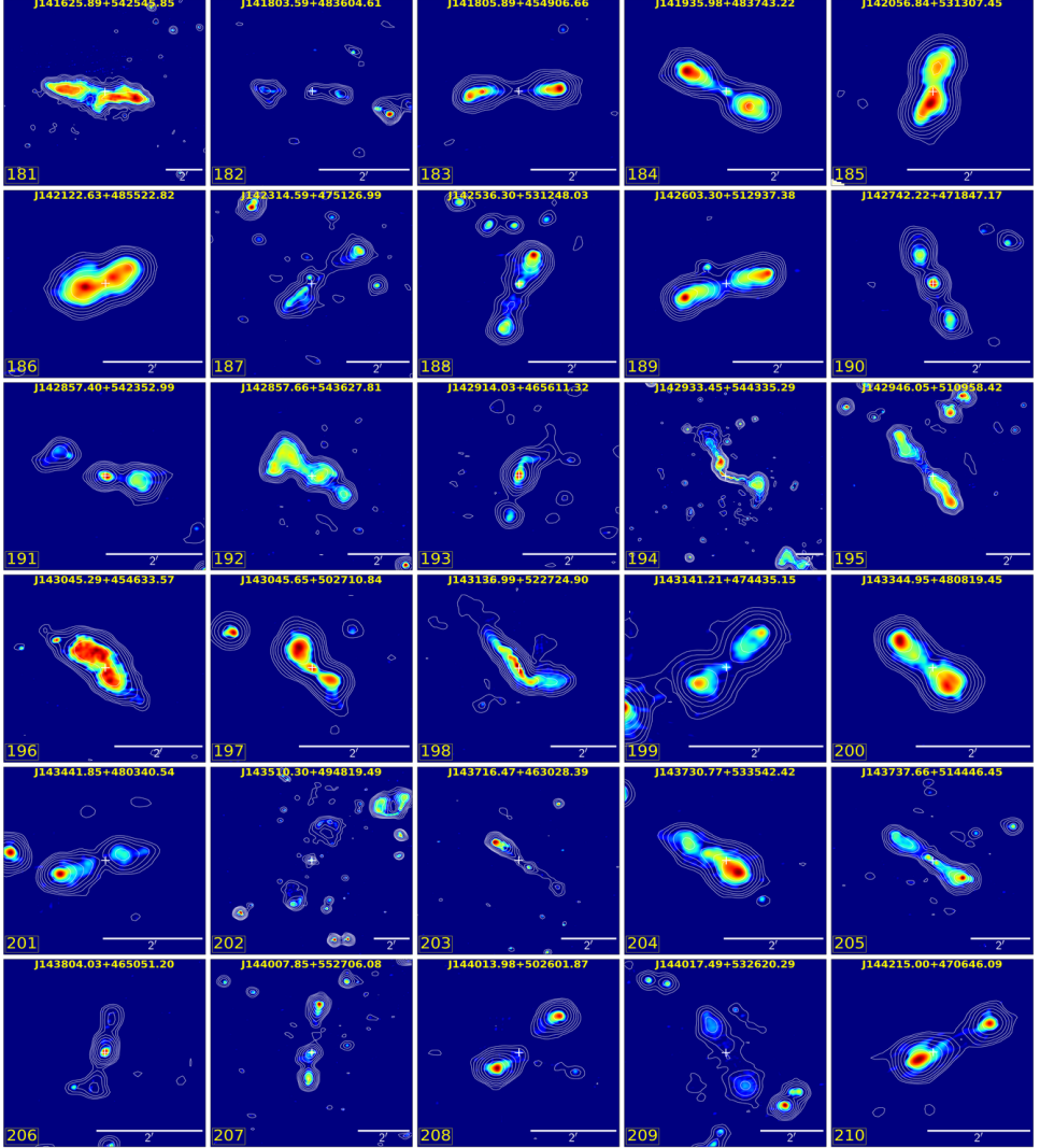
Figure 3.21: LoTSS high resolution ( \sim 6'' ) images 181-210 with LoTSS low resolution ( \sim 20'' ) contours overlaid. The cross '+' marker indicates the location of the host galaxy. The radio contours are drawn with 8 levels which are chosen by equally (log scale) dividing the data value range above \sim 3\sigma , where \sigma is the local RMS of the map.
