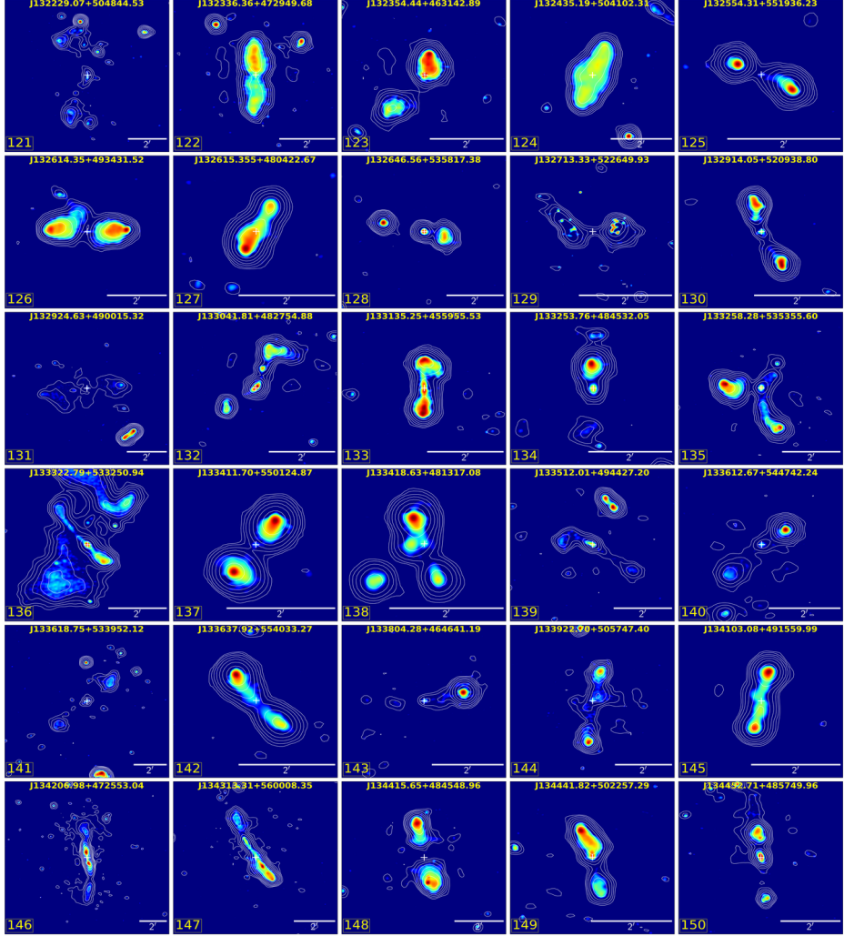
Figure 3.19: LoTSS high resolution ( \sim 6'' ) images 121-150 with LoTSS low resolution ( \sim 20'' ) contours overlaid. The cross '+' marker indicates the location of the host galaxy. The radio contours are drawn with 8 levels which are chosen by equally (log scale) dividing the data value range above \sim 3\sigma , where \sigma is the local RMS of the map.
