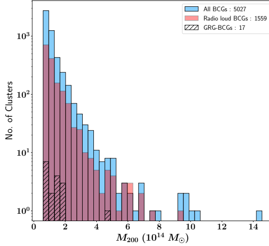
Figure 3.10: Distribution of M_{200} (mass of the cluster within r_{200} ) of clusters of galaxies.
