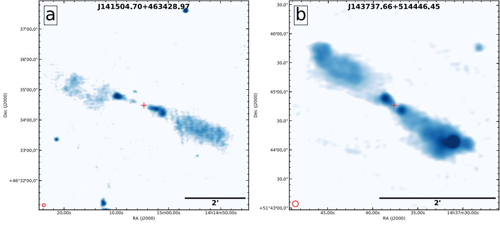
Figure 3.14: DDRGs postage-1 (13-14 DDRGs) made using LoTSS DR1 144 MHz radio image with 6'' \times 6'' resolution in inverted blue colour scale. Refer to Sect. 3.4.2 for more details.
