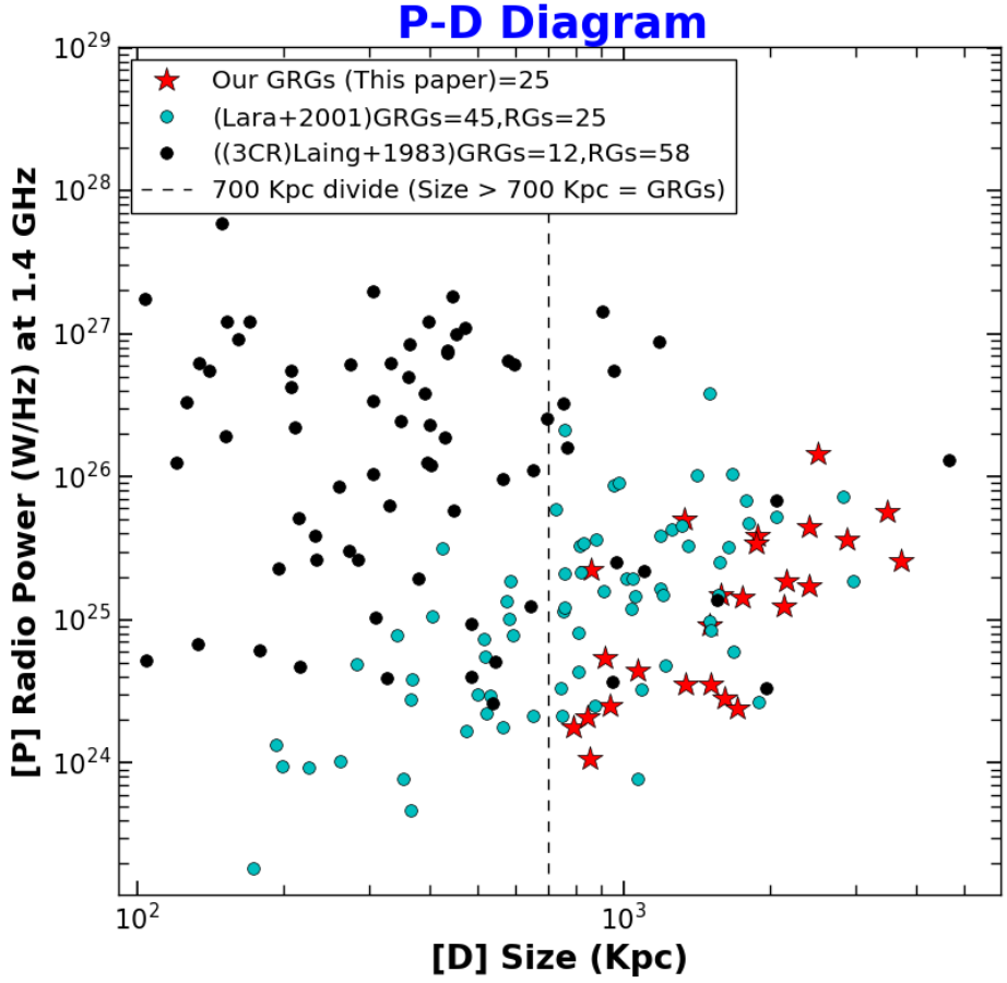
Figure 2.7: Above figure shows the newly discovered 25 GRGs plotted on the P-D diagram along with other known RGs and GRGs from different papers. Sizes and powers of known RGs and GRGs were recomputed for uniformity.
