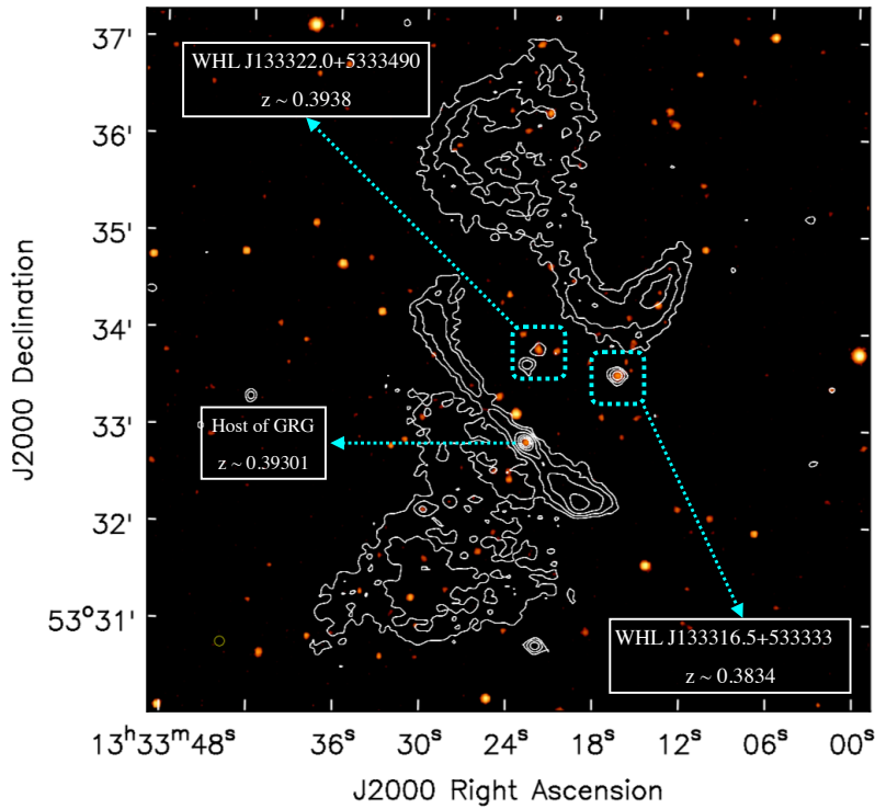
Figure 3.7: The figure shows GRG J133322.79+533250.94 amidst possibly galaxy cluster relics. The background image in orange colour is SDSS I band optical image which is superimposed with LoTSS DR1 high resolution ( 6'' ) contours.
