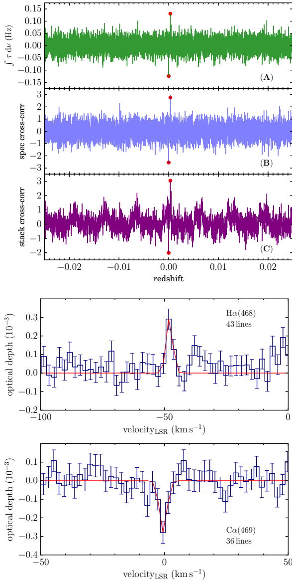
Figure 5.11: Left : Same as in Figure 5.8, except applied to C\alpha -transitions in Cas A spectra. Fits to the -47 \text{ km s}^{-1} and -38 \text{ km s}^{-1} components (and all higher order transitions) have been subtracted in the spectrum of Cas A. Residuals remaining from imperfect subtraction of the brightest \alpha transitions from -47 \text{ km s}^{-1} and -38 \text{ km s}^{-1} components can be seen in (C). These results demonstrate the behavior of the method in the presence of narrow, low signal-to-noise spectral lines. The redshifts ( z_H = 0.000337 and z_C = -0.000002 , with respect to stacking for C\alpha ) of the two detections are shown in red. Right : The stacked spectrum of H \alpha (top) associated with the -47 \text{ km s}^{-1} component, one of the lowest frequency detections of Hydrogen RRLs. Ca \alpha (bottom) associated with the Orion Arm, detected at this frequency for the first time.
