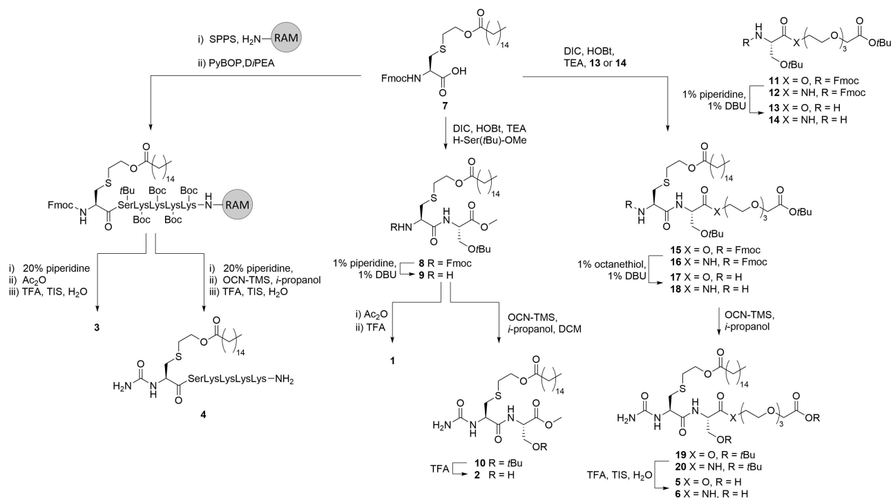
Scheme 1. Synthesis of TLR2 ligands 1–6 .
